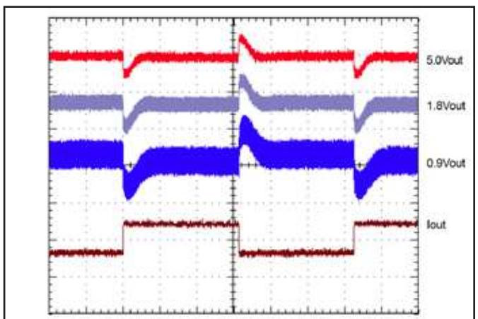
Figure 12: Output voltage response for 0.9V, 1.8V, 5V units to step-change in load current (50-75-50% of Iout max; di/dt=3A/us). Load cap: 470µF, 100mΩ ESR tant, 10µF cer. Ch 1: Iout (10A/div), Ch 2-4: Vout (100mV/div).
