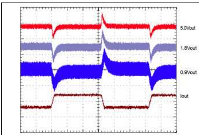
Figure 11: Output voltage response for 0.9V, 1.8V, 5V units to step-change in load current (50-75-50% of Iout max; di/dt=0.1A/us). Load cap: 100µF, 100mΩ ESR tant, 10µF cer. Ch 1: Iout (10A/div), Ch 2-4: Vout (100mV/div).
