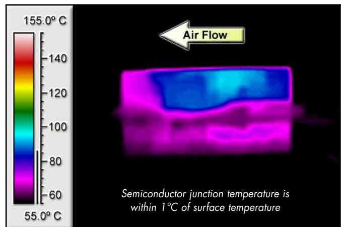
Figure 6: Thermal plot of 1.5Vo, 1.8Vo converters at nominal Vin and 16 amp load current mounted on a 55°C, 6-Layer, 2 oz. copper board (typical installation).
