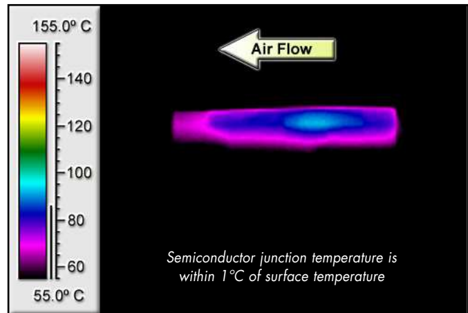
Figure 4: Thermal plot of 0.75Vo, 1.2Vo converters at nominal Vin and 16 amp load current mounted on a 55°C, 6-Layer, 2 oz. copper board (typical installation).
