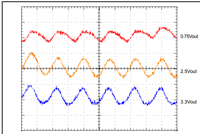
Figure 15: Input Terminal Ripple Voltage at nominal input voltage and rated load current (200 mV/div). Load capacitance: 22 F ceramic cap. Bandwidth: 20 MHz. See Figure 13.
