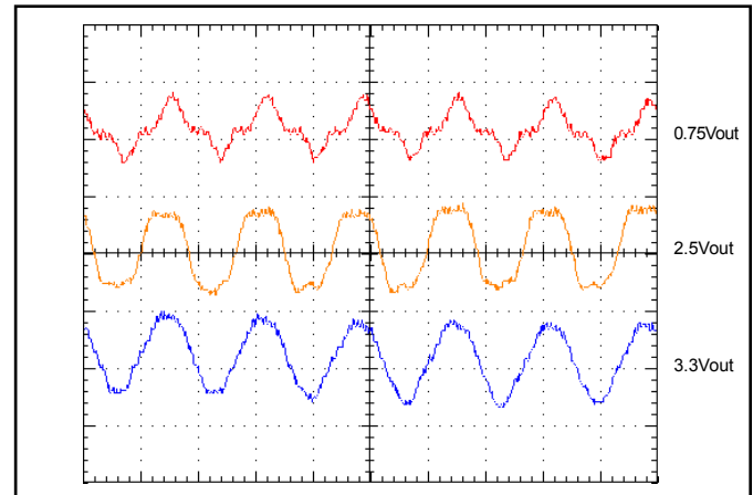
Figure 16: Output Voltage Ripple at nominal input voltage and rated load current (20 mV/div). Load capacitance: 22 F ceramic cap. Bandwidth: 20 MHz. See Figure 13.
