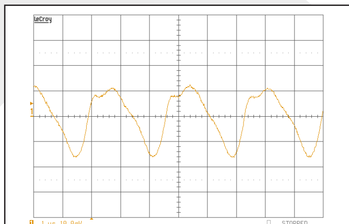
Figure 9: Input terminal current ripple, i_C , at full rated output current and nominal input voltage with SynQor MCOTS filter module (200 mA/div). Bandwidth: 25MHz. See Figure 17.
