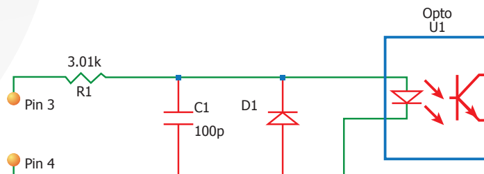
Figure B: Internal ON/OFF pin circuitry
