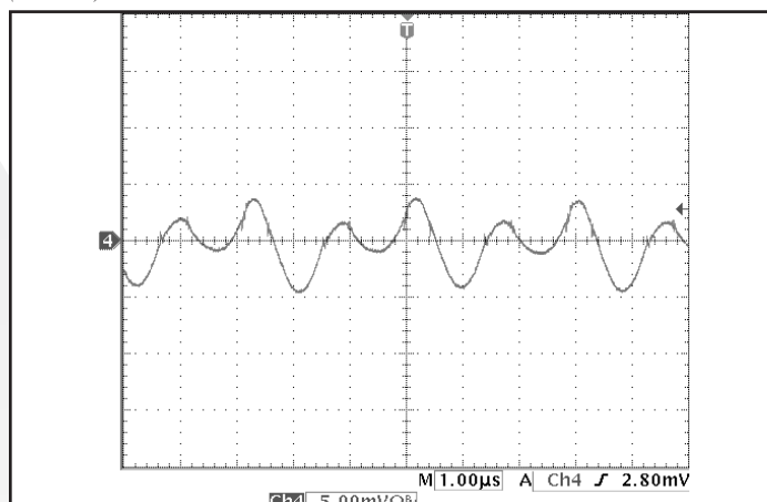
Figure 10: Output voltage ripple, Vout, at nominal input voltage and rated load current (5 mV/div). Load capacitance: 1μF ceramic capacitor and 10μF tantalum capacitor. Bandwidth: 10 MHz. See Figure 17.
