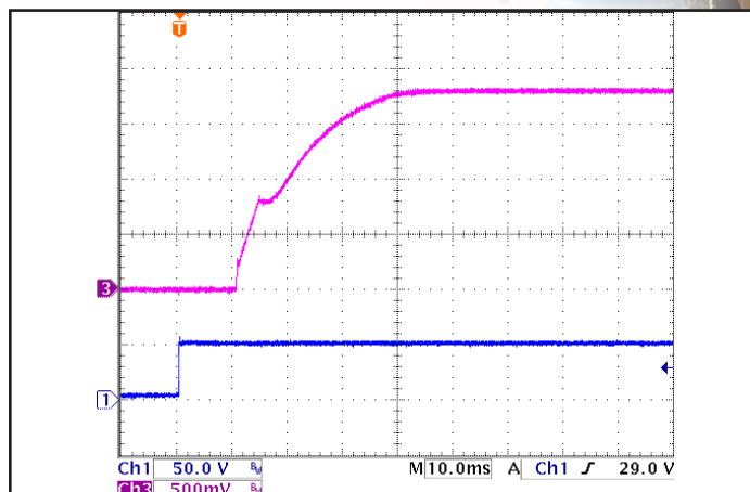
Figure 8: Turn-on transient at full resistive load and zero output capacitance initiated by Vin. ON/OFF Pin previously low. Ch 1: Vout (50V/div). Ch 3: Vin (0.5V/div).
