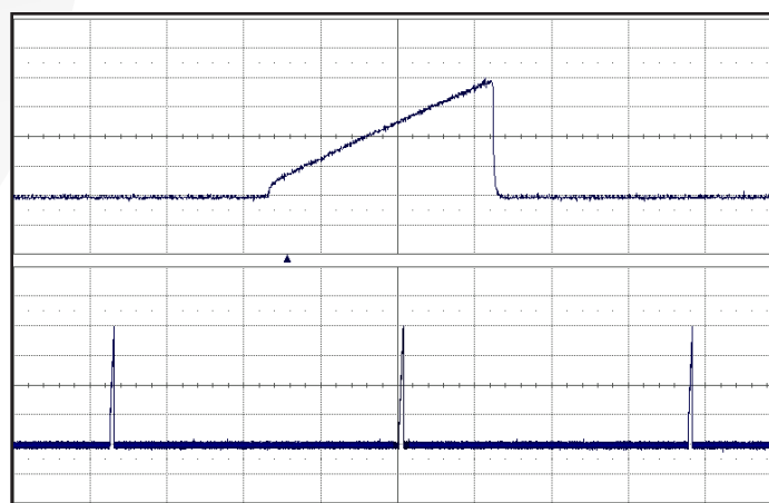
Figure 18: Load current (10A/div) as a function of time (2ms/div and 100ms/div) when the converter attempts to turn on into a 10 mΩ short circuit.
