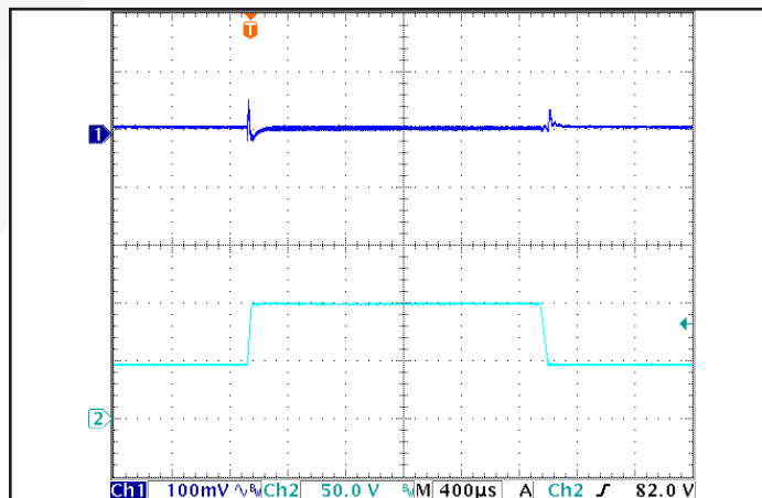
Figure 12: Output voltage response to step-change in input voltage (250V/ms). Load cap: 100 μF electrolytic output capacitance. Ch 1: Vout (100mV/div), Ch 2: Vin (50V/div).
