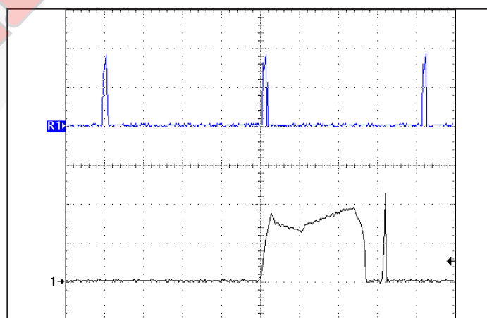
Figure 18: Load current (50A/div) as a function of time (2ms/div and 50ms/div) when the converter attempts to turn on into a 10 mΩ short circuit.
