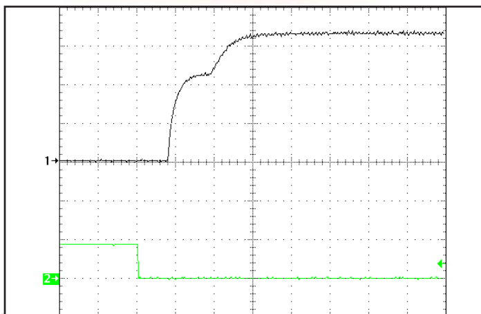
Figure 7: Typical startup waveform. Input voltage pre-applied, Ch 1: Vout (1V/div). Ch 2: ON/OFF (5V/div).
