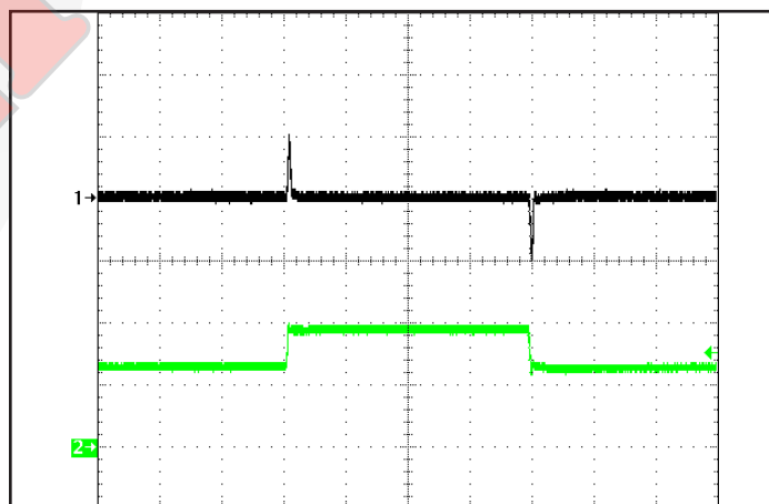
Figure 12: Output voltage response to step-change in input voltage (500V/ms) at full load current. Load cap: 100uf electrolytic capacitance. Ch1: Vout (.5V/div), Ch 2: Vin (20V/div).
