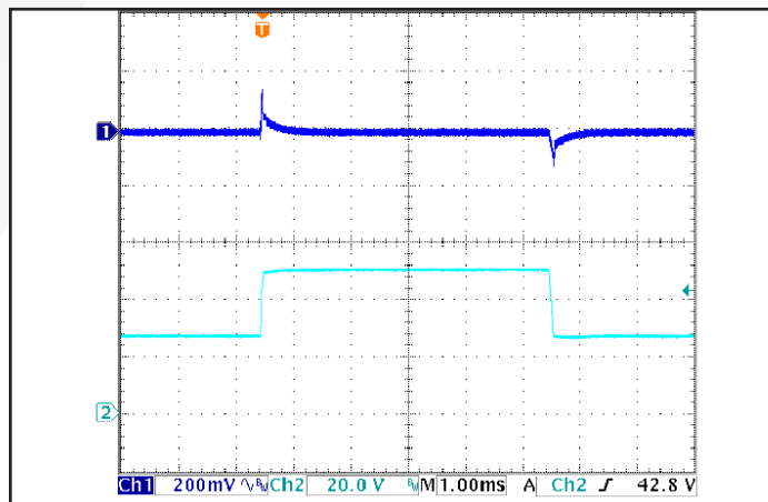
Figure 12: Output voltage response to step-change in input voltage (250V/ms). Load cap: 100 μF electrolytic output capacitance. Ch 1: Vout (200mV/div), Ch 2: Vin (20V/div).
