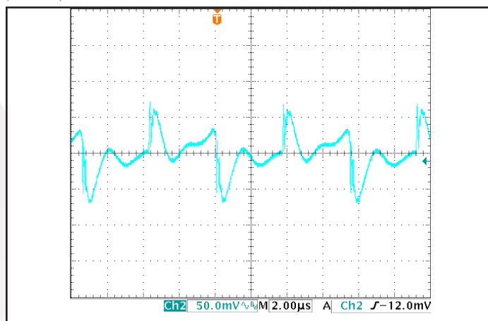
Figure 10: Output voltage ripple, Vout, at nominal input voltage and rated load current (50 mV/div). Load capacitance: 1μF ceramic capacitor and 10μF tantalum capacitor. Bandwidth: 10 MHz. See Figure 17.
