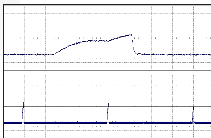
Figure 18: Load current (50A/div) as a function of time (1ms/div and 50ms/div) when the converter attempts to turn on into a 10 mΩ short circuit.
