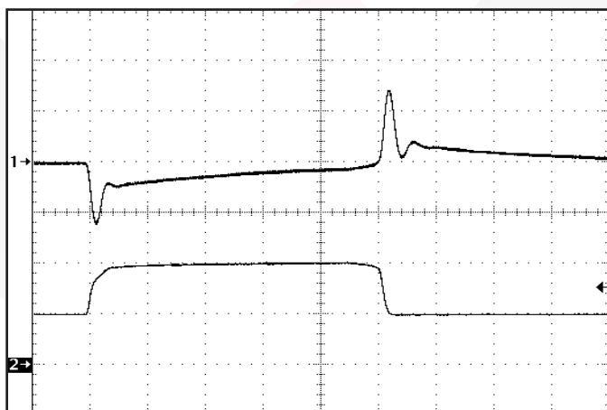
Figure 11: Output voltage response to step-change in load current 50%-100%-50% of Iout (max). Load cap: 1 \mu F ceramic cap and 10 \mu F, 100m \Omega ESR tantalum cap. Ch 1: Vout (200mV/div). Ch 2: Iout (20A/div).
