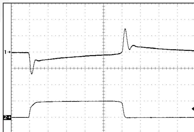
Figure 12: Output voltage response to step-change in load current 0%-50%-0% of Iout (max). Load cap: 1 \mu F ceramic cap and 10 \mu F, 100m \Omega ESR tantalum cap. Ch 1: Vout (200mV/div). Ch 2: Iout (20A/div).
