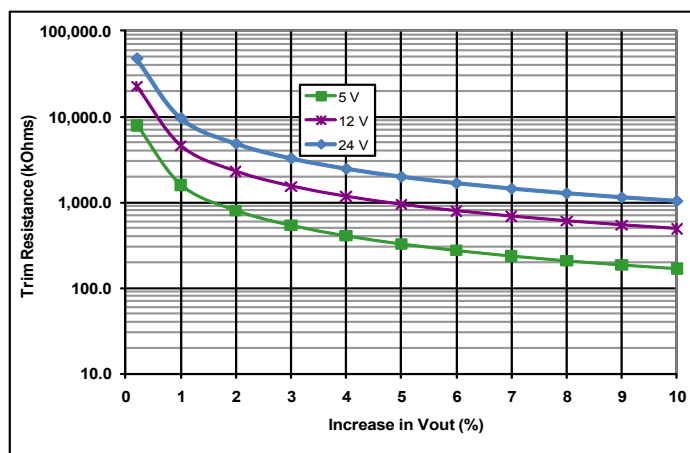
Common Figure 3: Trim graph for trim-up 5 to 24V outputs.
