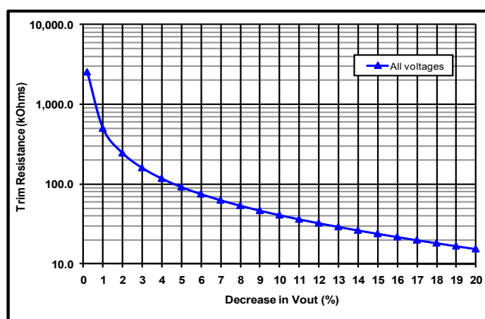
Common Figure 4: Trim graph for trim down.
