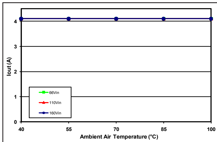
Figure 3: Encased Converter (no heatsink) max. output current derating vs. ambient air temperature for different Input Voltages and 0 LFM airflow (natural convection airflow).
