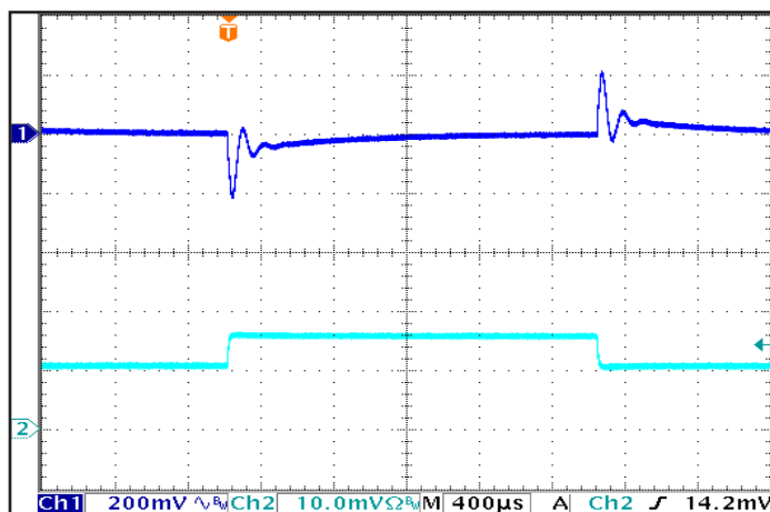
Figure 5: Output voltage response to step-change in load current (50%-75%-50% of Iout(max); dI/dt = 0.2 A/μs). Load cap: 1 μF ceramic and 15 μF tantalum capacitors. Ch 1: Vout, Ch 2: Iout (2A/div)
