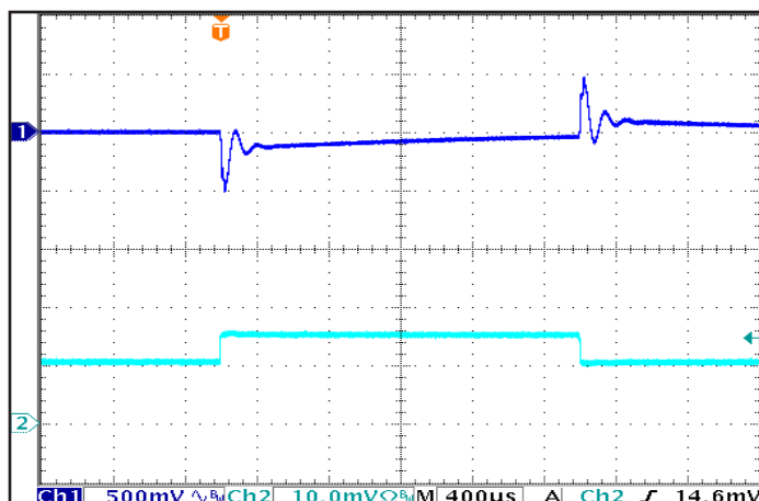
Figure 5: Output voltage response to step-change in load current (50%-75%-50% of I_{out(max)} ; dI/dt = 0.2 \text{ A}/\mu\text{s} ). Load cap: 1 \mu\text{F} ceramic capacitor. Ch 1: V_{out} , Ch 2: I_{out} (1A/div.)
