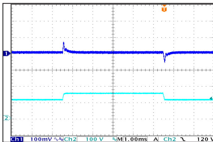
Figure 6: Output voltage response to step-change in input voltage (1000 V/ms). Load cap: 1 \mu\text{F} ceramic and 15 \mu\text{F} tantalum capacitors. Ch 1: V_{out} , Ch 2: V_{in} .
