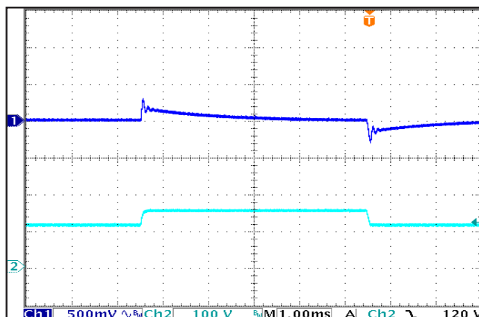
Figure 6: Output voltage response to step-change in input voltage (1000 V/ms). Load cap: 1 \mu\text{F} ceramic capacitor. Ch 1: V_{out} , Ch 2: V_{in} .
