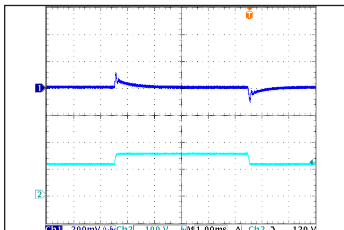
Figure 6: Output voltage response to step-change in input voltage (1000 V/ms). Load cap: 1 μF ceramic and 15 μF tantalum capacitors. Ch 1: Vout, Ch 2: Vin.
