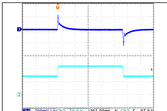
Figure 6: Output voltage response to step-change in input voltage (1000 V/ms, V_{nom}-V_{max}-V_{nom} ). Load cap: 1 \mu F ceramic and 15 \mu F tantalum capacitors. Ch 1: V_{out} , Ch 2: V_{in} .
