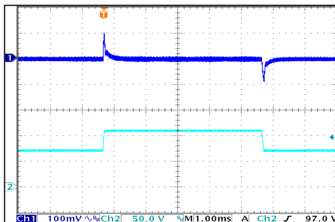
Figure 6: Output voltage response to step-change in input voltage (1000 V/ms, V_{nom}-V_{max}-V_{nom} ). Load cap: 1 \mu\text{F} ceramic and 15 \mu\text{F} tantalum capacitors. Ch 1: V_{out} , Ch 2: V_{in} .
