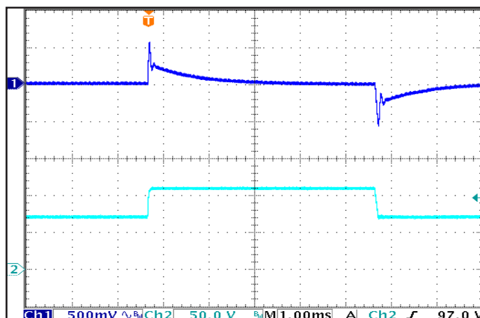
Figure 6: Output voltage response to step-change in input voltage (1000 V/ms, V_{nom}-V_{max}-V_{nom} ). Load cap: 1 \mu F ceramic capacitor. Ch 1: V_{out} , Ch 2: V_{in} .
