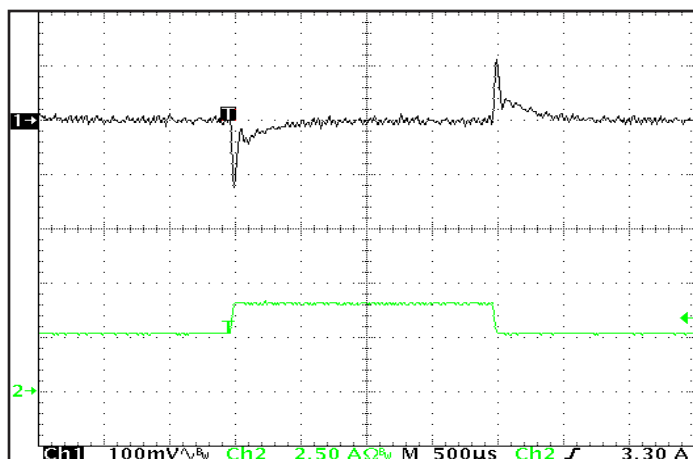
Figure 5: Output voltage response to step-change in load current (50%-75%-50% of Iout(max); dI/dt = 0.05A/μs. Load cap: 15μF tantalum cap and 1μF ceramic cap. Ch 1: Vout, Ch 2: Iout.
