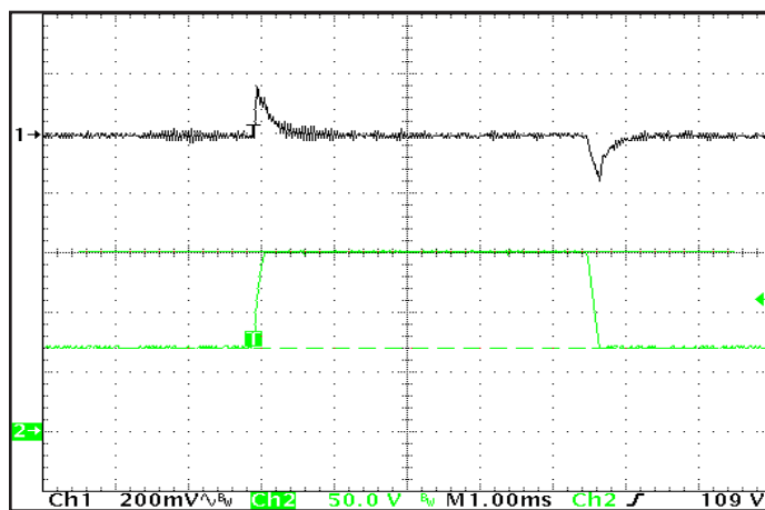
Figure 6: Output voltage response to step-change in input voltage (715V/ms), at Max. load current. Load cap: 15μF tantalum cap and 1μF ceramic cap. Ch 1: Vout, Ch 2: Vin.
