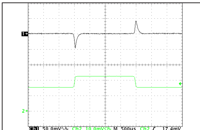
Figure 5: Output voltage response to step-change in load current (50%-75%-50% of Iout(max); dI/dt = 0.1A/μs). Load cap: 15μF, 100 mΩ ESR tantalum cap and 1μF ceramic cap. Ch 1: Vout (50mV/div), Ch 2: Iout (10A/div).
