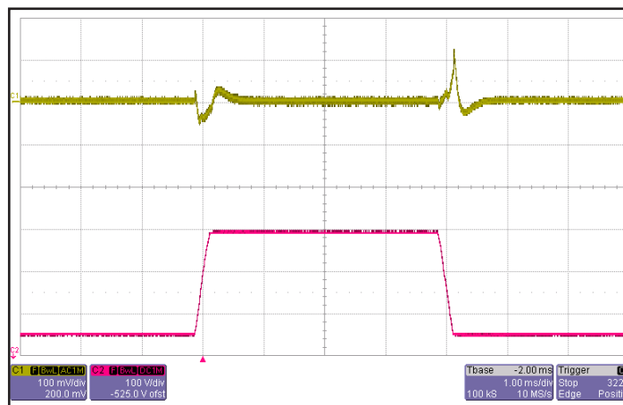
Figure 6: Output voltage response to step-change in input voltage (180 V - 425 V - 180 V) with 250 μs rise/fall time. Load cap: 15μF, 100 mΩ ESR tantalum cap and 1μF ceramic cap. Ch 1: Vout (100mV/div). Ch 2: Vin (100V/div).
