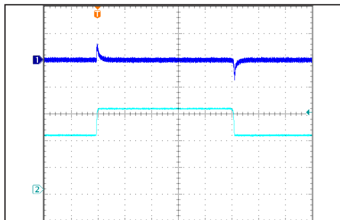
Figure 6: Output voltage response to step-change in input voltage (72V to 100V), at 25A load current. Load cap: 15μF tantalum capacitor and 1μF ceramic cap. Ch 1: V out (100mV/div), Ch 2: V in (50V/div).
