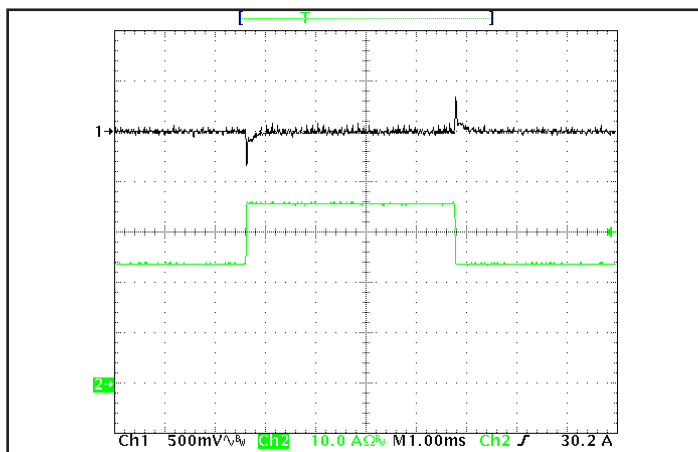
Figure 5: Output voltage response to step-change in load current (70%-100%-70% of I_{out(max)} ; dI/dt = 0.1A/\mu s . Load cap: 15 \mu F tantalum cap and 1 \mu F ceramic cap. Ch 1: V_{out} , Ch 2: I_{out} (10 A/div).
