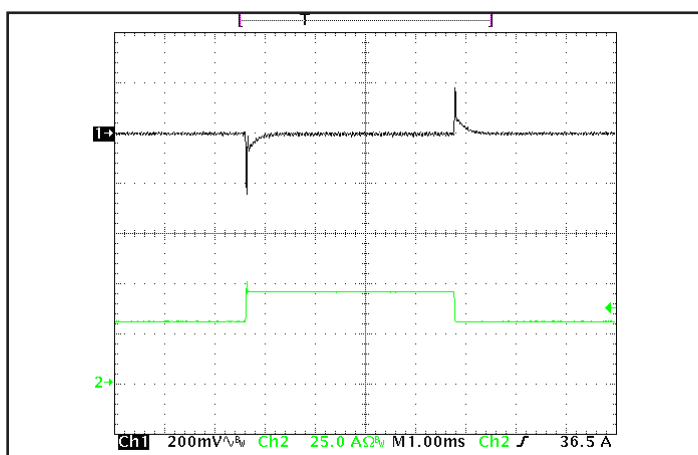
Figure 5: Output voltage response to step-change in load current (65%-100%-65% of Iout(max); dI/dt = 0.1A/μs). Load cap: 15μF tantalum cap and 1μF ceramic cap. Ch 1: Vout, Ch 2: Iout (25 A/div).
