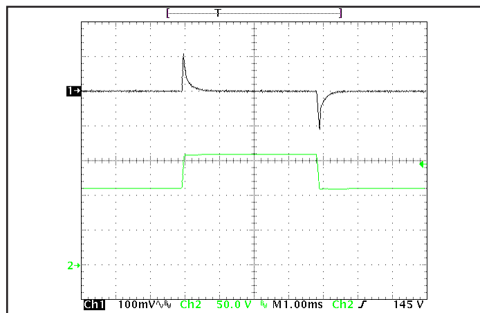
Figure 6: Output voltage response to step-change in input voltage (1000 V/ms), at Max. load current. Load cap: 15 \mu F tantalum cap and 1 \mu F ceramic cap. Ch 1: V_{out} , Ch 2: V_{in} .
