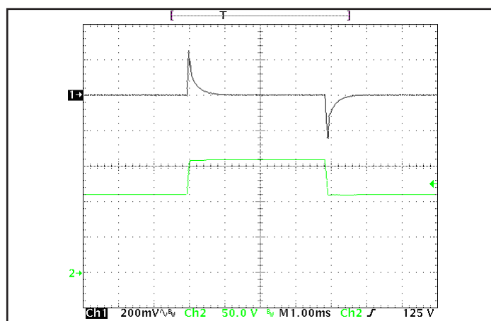
Figure 6: Output voltage response to step-change in input voltage (1000 V/ms), at Max. load current. Load cap: 15μF tantalum cap and 1μF ceramic cap. Ch 1: V out , Ch 2: V in .
