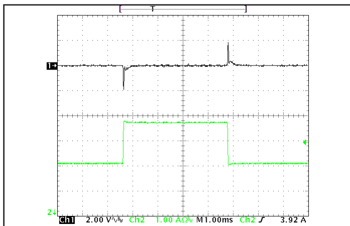
Figure 5: Output voltage response to step-change in load current (65%-95%-65% of I out (max); dI/dt = 0.1A/μs. Load cap: 1μF ceramic cap. Ch 1: V out , Ch 2: I out (1 A/div).
