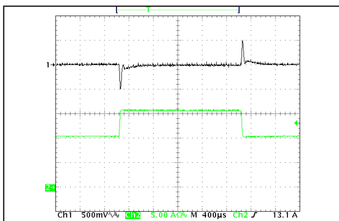
Figure 5: Output voltage response to step-change in load current (65%-100%-65% of I out (max); dI/dt = 0.1A/μs. Load cap: 15μF tantalum cap and 1μF ceramic cap. Ch 1: V out , Ch 2: I out (5 A/div).
