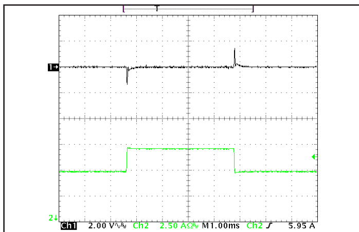
Figure 5: Output voltage response to step-change in load current (65%-95%-65% of I out (max); dI/dt = 0.1A/μs. Load cap: 1μF ceramic cap. Ch 1: V out , Ch 2: I out (2.5 A/div).
