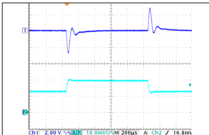
Figure 5: Output voltage response to step-change in load current (65%-100%-65% of I out (max); dI/dt = 0.1A/μs. Load cap: 1μF ceramic cap. Ch 1: V out , Ch 2: I out (2 A/div).
