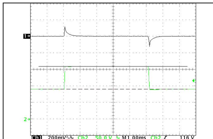
Figure 6: Output voltage response to step-change in input voltage (nominal to maximum), at full load current. Load cap: 15μF tantalum capacitor and 1μF ceramic cap. Ch 1: V out , Ch 2: V in .
