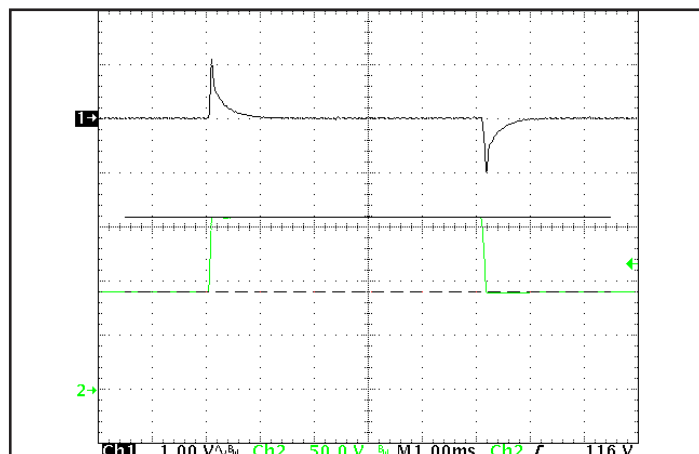
Figure 6: Output voltage response to step-change in input voltage (nominal to maximum), at full load current. Load cap: 1uF ceramic cap. Ch 1: V out , Ch 2: V in .
