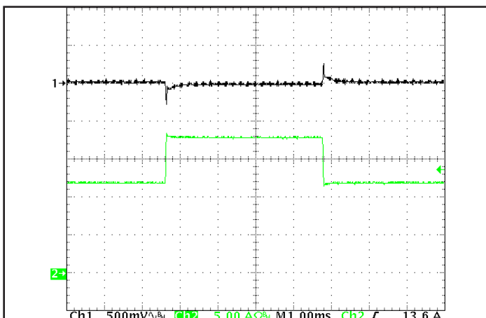
Figure 5: Output response to load current step for QTC version of product (50%-75%-50% of I out (max); dI/dt = 0.1A/μs). Load cap: 15μF tantalum cap and 1μF ceramic cap. Ch 1: V out , Ch 2: I out .
