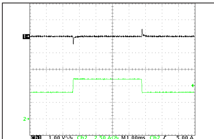
Figure 5: Output voltage response to step-change in load current (75%-100%-75% of Iout(max); dI/dt = 0.1A/μs). Load cap: 15μF tantalum cap and 1μF ceramic cap. Ch 1: Vout, Ch 2: Iout.
