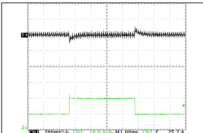
Figure 5: Output voltage response to step-change in load current (65%-95%-65% of Iout(max); dI/dt = 0.1A/μs). Load cap: 15μF tantalum cap and 1μF ceramic cap. Ch 1: Vout, Ch 2: Iout.
