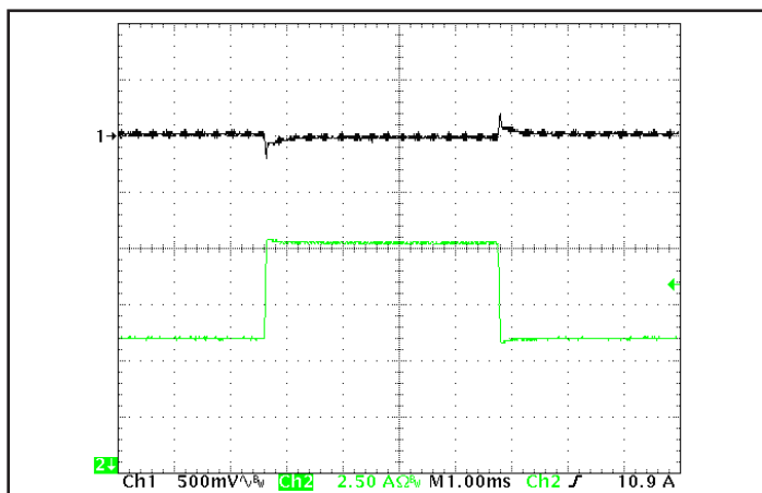
Figure 5: Output voltage response to step-change in load current (50%-75%-50% of Iout(max); dI/dt = 0.1A/\mu s ). Load cap: 15 \mu F tantalum cap and 1 \mu F ceramic cap. Ch 1: Vout, Ch 2: Iout.
