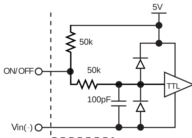
Figure B: Internal ON/OFF pin circuitry
