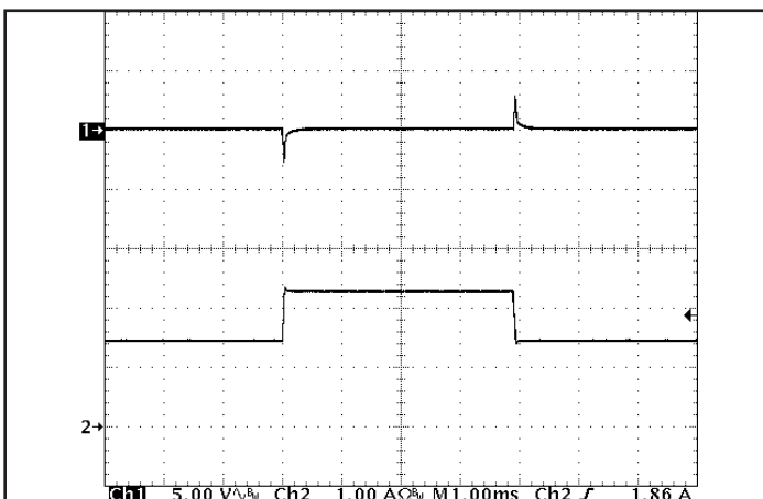
Figure 5: Output voltage response to step-change in load current (50%-75%-50% of I out (max); dI/dt = 0.2 A/μs). Load cap: 1 μF ceramic capacitor. Ch 1: V out , Ch 2: I out .
