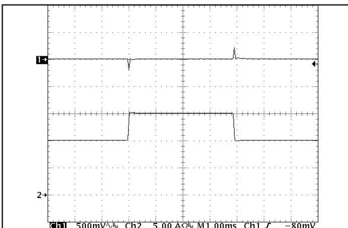
Figure 5: Output voltage response to step-change in load current (50%-75%-50% of Iout(max); dI/dt = 0.2 A/μs). Load cap: 1 μF ceramic and 15 μF tantalum capacitors. Ch 1: Vout, Ch 2: Iout.
