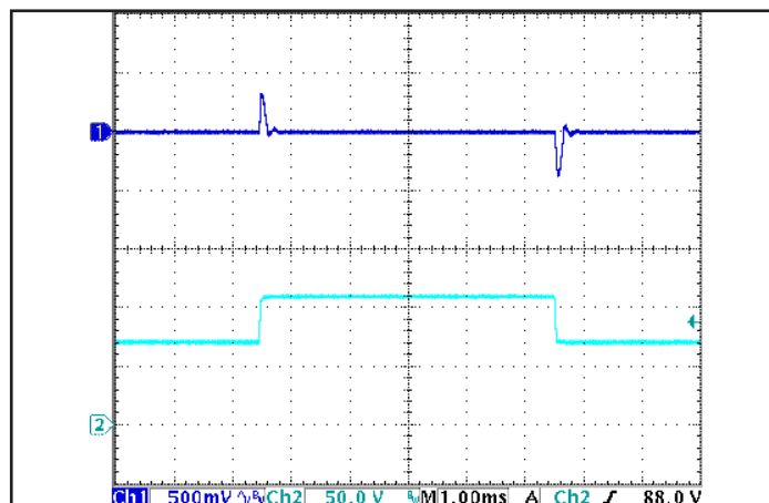
Figure 6: Output voltage response to step-change in input voltage (1000 V/ms). Load cap: 100 μF, electrolytic output capacitance. Ch 1: V out (500 mV/div), Ch 2: V in (50 V/div).
