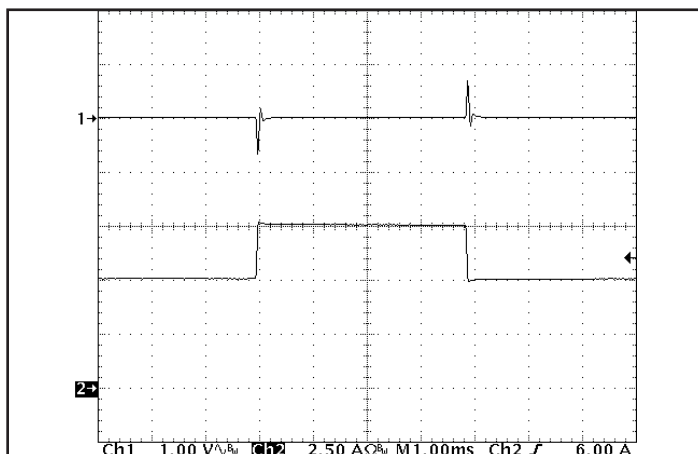
Figure 5: Output voltage response to step-change in load current (66%-100%-66% of I out (max); dI/dt = 0.1 A/μs). Load cap: 1 μF ceramic and 15 μF tantalum capacitors. Ch 1: V out (1 V/div), Ch 2: I out (2.5 A/div).
