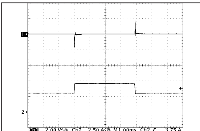
Figure 5: Output voltage response to step-change in load current (66%-100%-66% of I out (max); dI/dt = 0.08 A/μs). Load cap: 1 μF ceramic capacitor. Ch 1: V out (2 V/div), Ch 2: I out (2.5 A/div).
