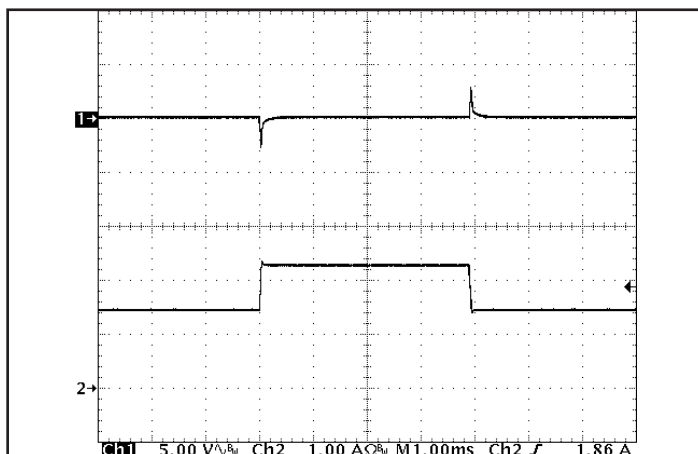
Figure 5: Output voltage response to step-change in load current (566%-100%-66% of Iout(max); dI/dt = 0.02 A/μs). Load cap: 1 μF ceramic capacitor. Ch 1: Vout (5 V/div), Ch 2: Iout (1 A/div).
