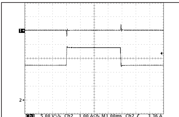
Figure 5: Output voltage response to step-change in load current (66%-100%-66% of I out (max); dI/dt = 0.05 A/μs). Load cap: 1 μF ceramic capacitor. Ch 1: V out (5 V/div), Ch 2: I out (1 A/div).
