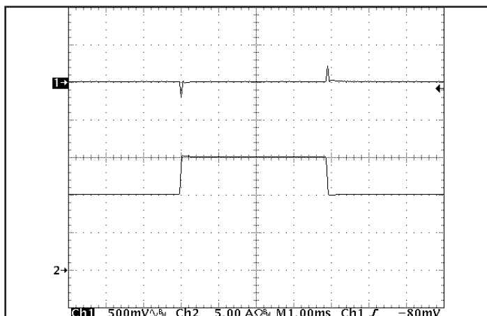
Figure 5: Output voltage response to step-change in load current (66%-100%-66% of I out (max); dI/dt = 0.1 A/μs). Load cap: 1 μF ceramic and 15 μF tantalum capacitors. Ch 1: V out (500 mV/div), Ch 2: I out (5 A/div).
