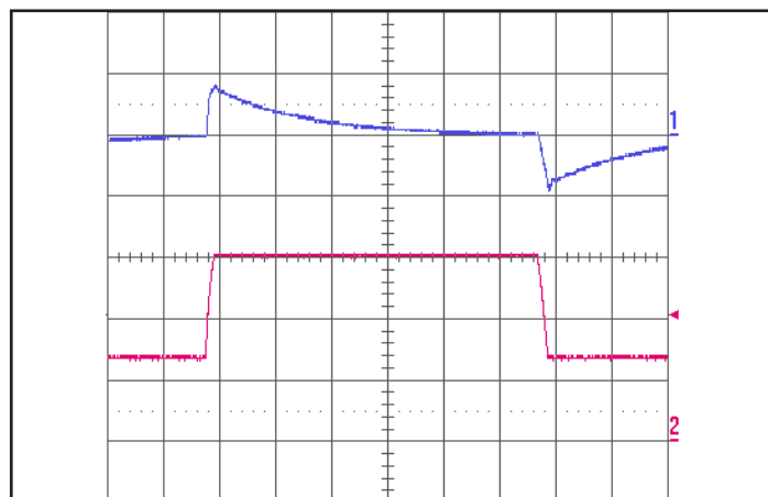
Figure 6: Output voltage response to step-change in input voltage (600 V/ms), at Max. load current. Load cap: 1μF ceramic cap. Ch 1: V out (2V/div), Ch 2: V in (50V/div), time scale: 1ms/div.
