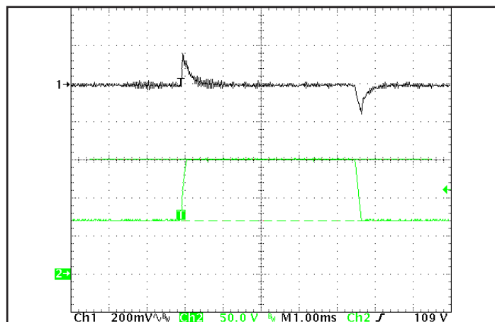
Figure 6: Output voltage response to step-change in input voltage (715V/ms), at Max. load current. Load cap: 15μF tantalum cap and 1μF ceramic cap. Ch 1: Vout, Ch 2: Vin.
