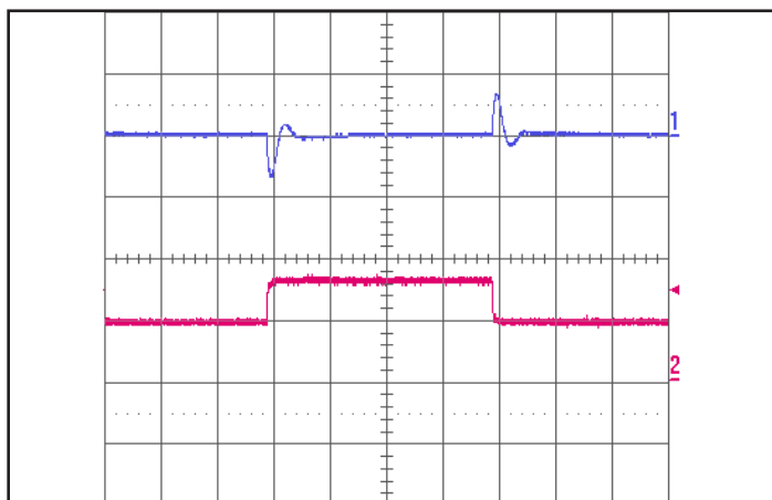
Figure 5: Output voltage response to step-change in load current (50%-75%-50% of Iout(max); dI/dt = 0.02A/μs. Load cap: 1μF ceramic cap. Ch 1: Vout (1V/div), Ch 2: Iout (500mA/div), time scale: 500μs/div.
