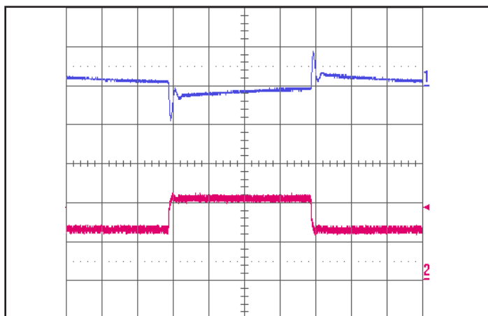
Figure 5: Output voltage response to step-change in load current (50%-75%-50% of I out (max); dI/dt = 0.01A/μs. Load cap: 1μF ceramic cap. Ch 1: V out (1V/div), Ch 2: I out (200mA/div), time scale: 500μs/div.
