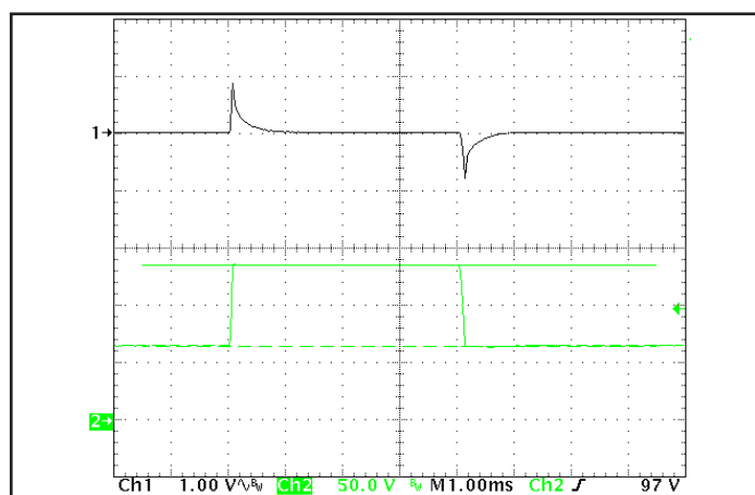
Figure 6: Output voltage response to step-change in input voltage (1000 V/ms). Load cap: 1 μF ceramic capacitor. Ch 1: Vout, Ch 2: Vin.
