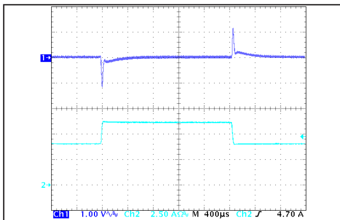
Figure 5: Output voltage response to step-change in load current (50%-75%-50% of I_{out(max)} ; dI/dt = 0.1 \text{ A}/\mu\text{s} ). Load cap: 1 \mu\text{F} ceramic capacitor. Ch 1: V_{out} (1 V/div), Ch 2: I_{out} (2.5 A/div).
