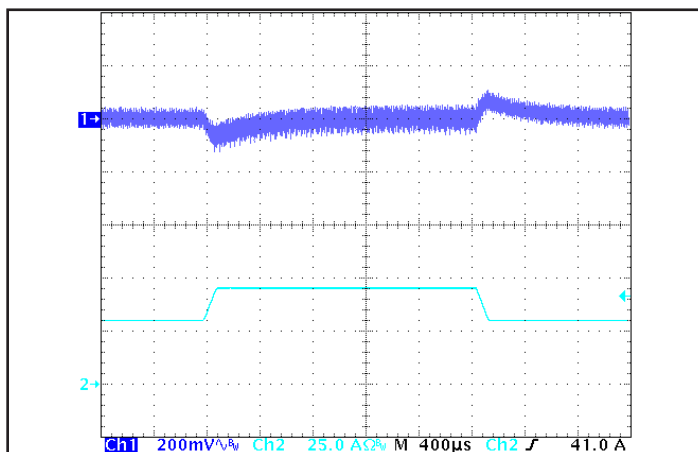
Figure 5: Output voltage response to step-change in load current (50%-75%-50% of I out (max); dI/dt = 0.1 A/μs). Load cap: 15 μF Tantalum+ 1 μF ceramic capacitor. Ch 1: V out (200 mV/div), Ch 2: I out (25 A/div).
