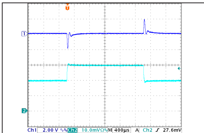
Figure 5: Output voltage response to step-change in load current (50%-75%-50% of I out(max) ; dI/dt = 0.1 A/μs). Load cap: 1 μF ceramic capacitor. Ch 1: V out (2 V/div), Ch 2: I out (1 A/div).
