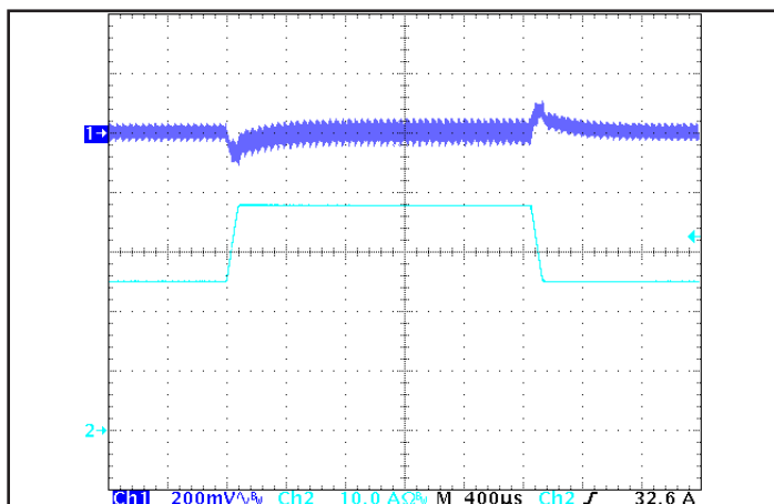
Figure 5: Output voltage response to step-change in load current (50%-75%-50% of I out (max); dI/dt = 0.1 A/μs). Load cap: 15 μF Tantalum + 1 μF ceramic capacitor. Ch 1: V out (200 mV/div), Ch 2: I out (10 A/div).
