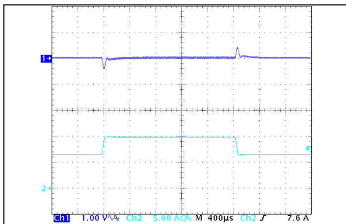
Figure 5: Output voltage response to step-change in load current (50%-75%-50% of I out (max); dI/dt = 0.1 A/μs). Load cap: 15 μF Tantalum + 1 μF ceramic capacitor. Ch 1: V out (1 V/div), Ch 2: I out (5 A/div).
