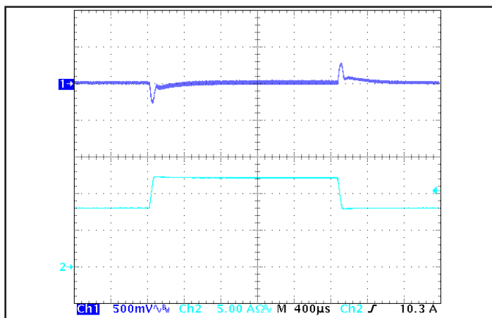
Figure 5: Output voltage response to step-change in load current (50%-75%-50% of I out (max); dI/dt = 0.1 A/μs). Load cap: 15 μF Tantalum + 1 μF ceramic capacitor. Ch 1: V out (500 mV/div), Ch 2: I out (5 A/div).
