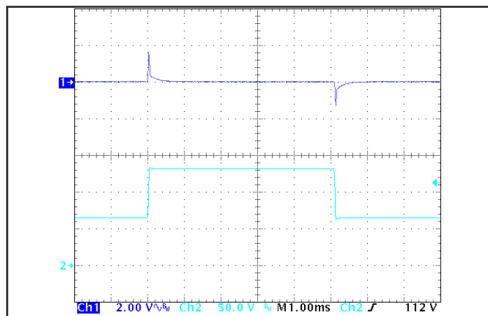
Figure 6: Output voltage response to step-change in input voltage (1000 V/ms). Load cap: 100 \mu\text{F} electrolytic output capacitance. Ch 1: V_{out} (2 V/div), Ch 2: V_{in} (50 V/div).
