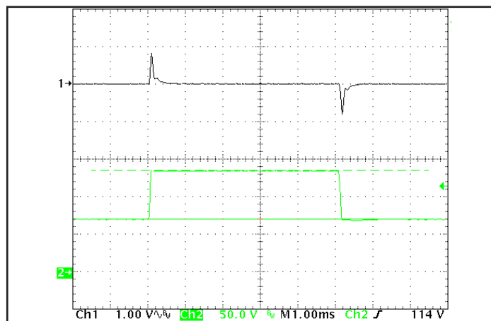
Figure 6: Output voltage response to step-change in input voltage (nominal to maximum), at full load current. Load cap: 1uF ceramic cap. Ch 1: Vout, Ch 2: Vin.
