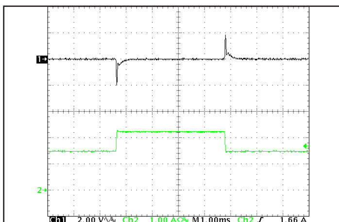
Figure 5: Output voltage response to step-change in load current (66%-100%-66% of Iout(max); dI/dt = 0.1A/μs). Load cap: 15μF tantalum cap and 1μF ceramic cap. Ch 1: Vout, Ch 2: Iout.
