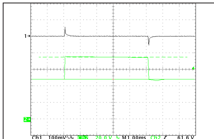
Figure 6: Output voltage response to step-change in input voltage (nominal to maximum input voltage), at 25A load current. Load cap: 15μF tantalum capacitor and 1uF ceramic cap. Ch 1: Vout, Ch 2: Vin.
