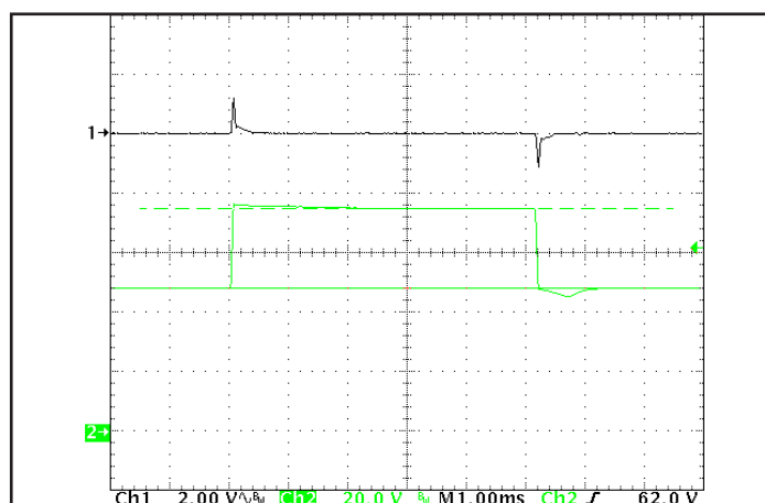
Figure 6: Output voltage response to step-change in input voltage (nominal to maximum input voltage), at 25A load current. Load cap: uF ceramic cap. Ch 1: Vout, Ch 2: Vin.
