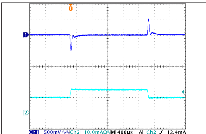
Figure 5: Output voltage response to step-change in load current (66%-100%-66% of Iout(max); dI/dt = 0.1A/μs). Load cap: 15μF tantalum cap and 1μF ceramic cap. Ch 1: Vout, Ch 2: Iout.
