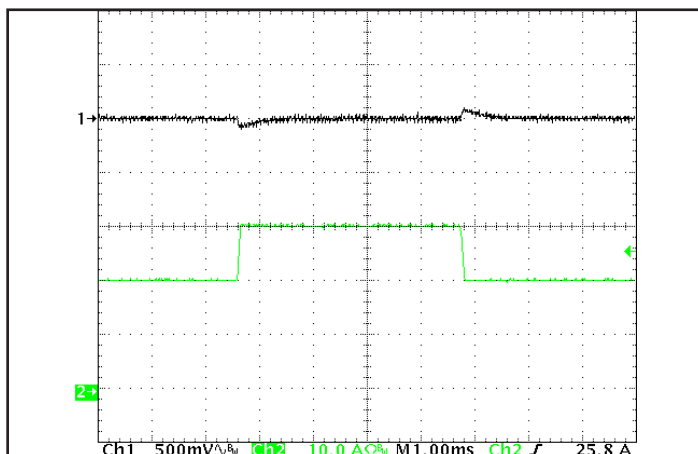
Figure 5: Output voltage response to step-change in load current (66%-100% of Iout(max); dI/dt = 0.1A/μs). Load cap: 15μF tantalum cap and 1μF ceramic cap. Ch 1: Vout, Ch 2: Iout.
