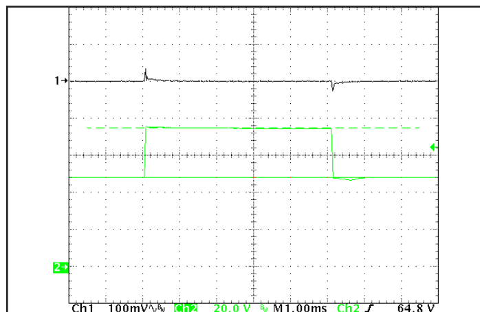
Figure 6: Output voltage response to step-change in input voltage (nominal to maximum input voltage), at 25A load current. Load cap: 15μF tantalum capacitor and 1μF ceramic cap. Ch 1: Vout, Ch 2: Vin.
