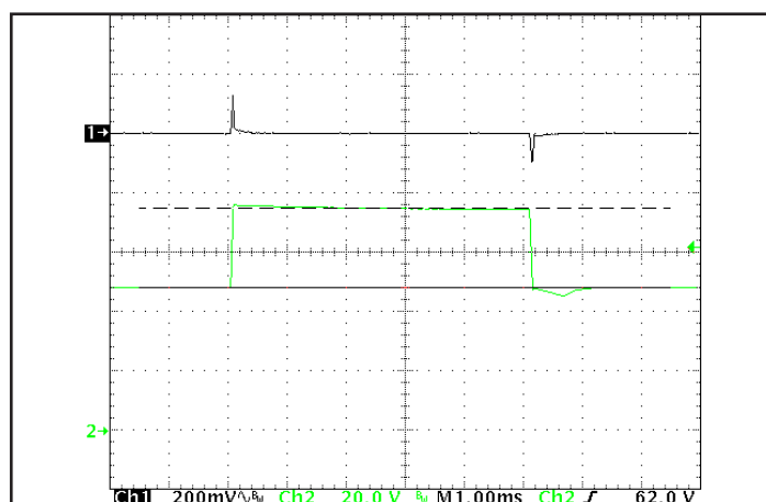
Figure 6: Output voltage response to step-change in input voltage (nominal to maximum input voltage), at 25A load current. Load cap: 15μF tantalum capacitor and 1μF ceramic cap. Ch 1: Vout, Ch 2: Vin.
