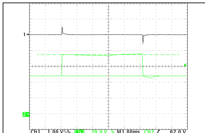
Figure 6: Output voltage response to step-change in input voltage (nominal to maximum input voltage), at 25A load current. Load cap: uF ceramic cap. Ch 1: Vout, Ch 2: Vin.
