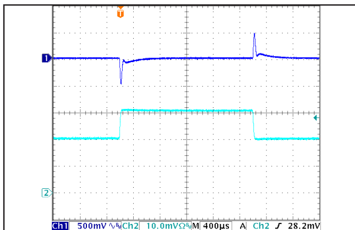
Figure 5: Output voltage response to step-change in load current (50%-75%-50% of I out (max); dI/dt = 0.1 A/μs). Load cap: 15 μF Tantalum + 1 μF Ceramic capacitor. Ch 1: V out , Ch 2: I out (5A/div).
