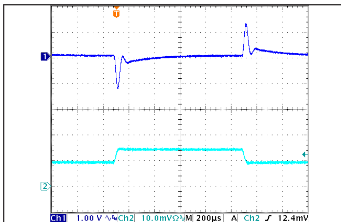
Figure 5: Output voltage response to step-change in load current (50%-75%-50% of I out (max); dI/dt = 0.1 A/μs). Load cap: 1 μF Ceramic capacitor. Ch 1: V out , Ch 2: I out (5A/div).
