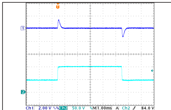
Figure 6: Output voltage response to step-change in input voltage (1000 V/ms). Load cap: 1 \mu F Ceramic capacitor. Ch 1: V_{out} , Ch 2: V_{in} .
