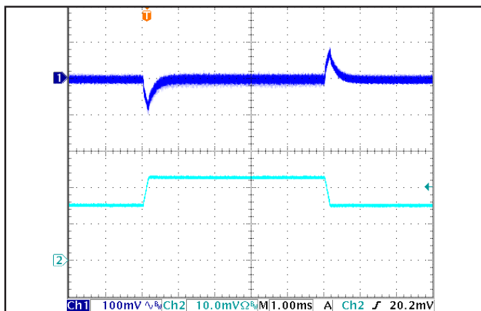
Figure 5: Output voltage response to step-change in load current (50%-75%-50% of Iout(max); dI/dt = 0.1 A/μs). Load cap: 15 μF Tantalum + 1 μF Ceramic capacitor. Ch 1: Vout, Ch 2: Iout (10A/div).
