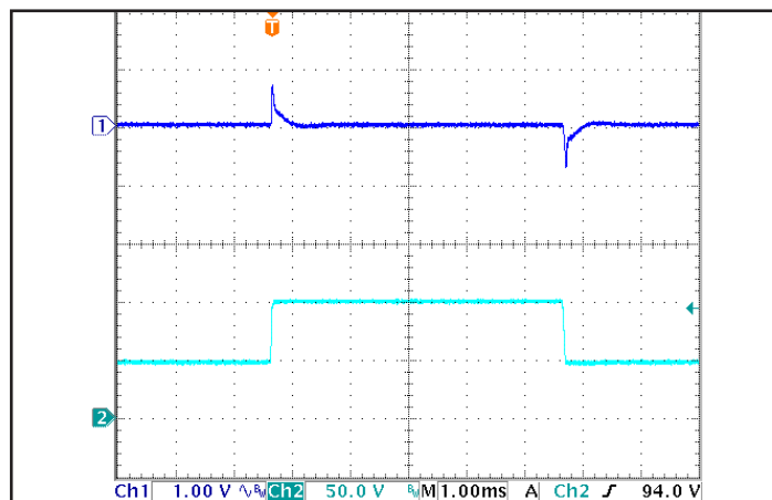
Figure 6: Output voltage response to step-change in input voltage (1000 V/ms). Load cap: 15 μF Tantalum + 1 μF Ceramic capacitor. Ch 1: V out , Ch 2: V in .
