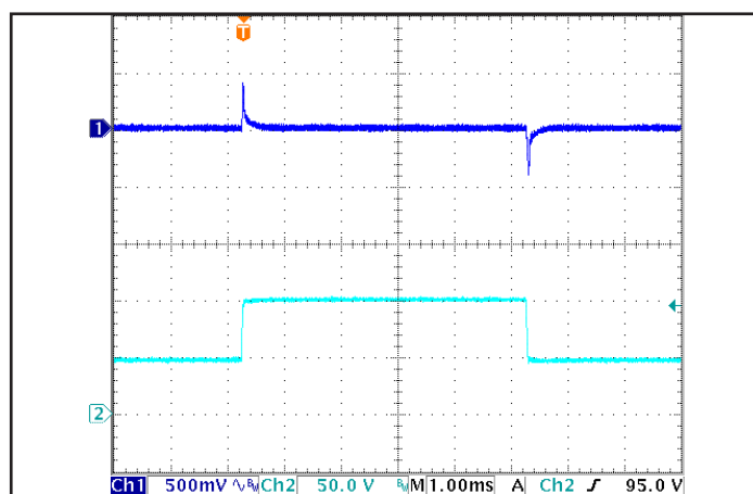
Figure 6: Output voltage response to step-change in input voltage (1000 V/ms). Load cap: 15 μF Tantalum + 1 μF Ceramic capacitor. Ch 1: V out , Ch 2: V in .
