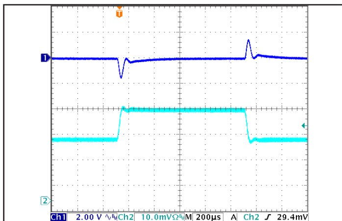
Figure 5: Output voltage response to step-change in load current (50%-75%-50% of I out (max); dI/dt = 0.1 A/μs). Load cap: 1 μF Ceramic capacitor. Ch 1: V out , Ch 2: I out (2A/div).
