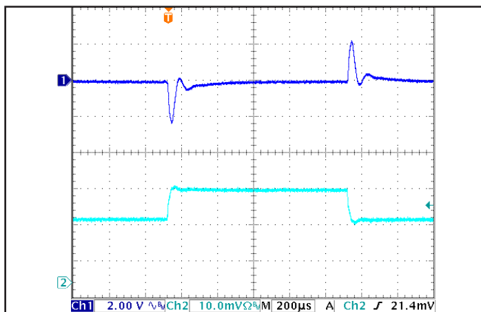
Figure 5: Output voltage response to step-change in load current (50%-75%-50% of I_{out(max)} ; dI/dt = 0.1 A/\mu s ). Load cap: 1 \mu F Ceramic capacitor. Ch 1: V_{out} , Ch 2: I_{out} (2A/div).
