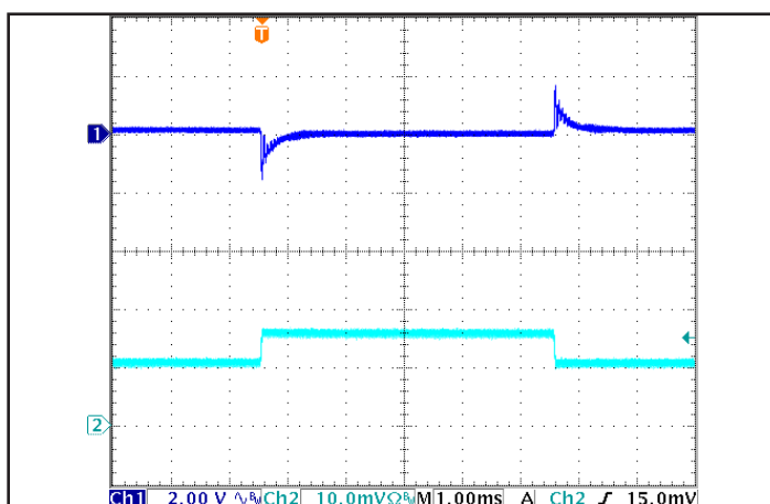
Figure 5: Output Voltage Response to Step-Change in Load Current (50%-75%-50% of Iout(max); dI/dt = 0.1A/μs. Load cap: 1μF ceramic cap. Ch 1: Vout, Ch 2: Iout (5 A/div).
