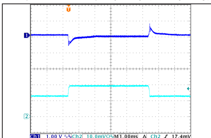
Figure 5: Output Voltage Response to Step-Change in Load Current (50%-75%-50% of I out (max); dI/dt = 0.1A/μs. Load cap: 15μF tantalum cap and 1μF ceramic cap. Ch 1: V out , Ch 2: I out (10 A/div).
