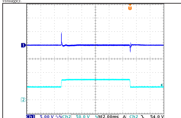
Figure 6: Output Voltage Response to Step-Change in Input Voltage (500 V/ms), at Max. load current. Load cap: 100μF electrolytic cap and 1μF ceramic cap. Ch 1: V out , Ch 2: V in .
