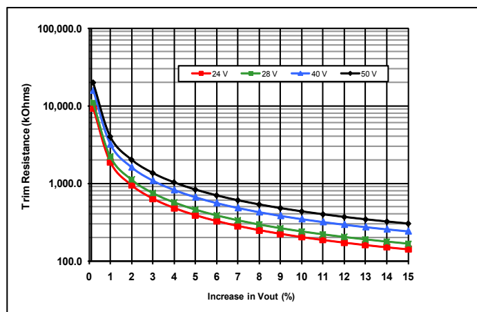
Common Figure 4: Trim-Up Graph for 24 to 50V outputs.
