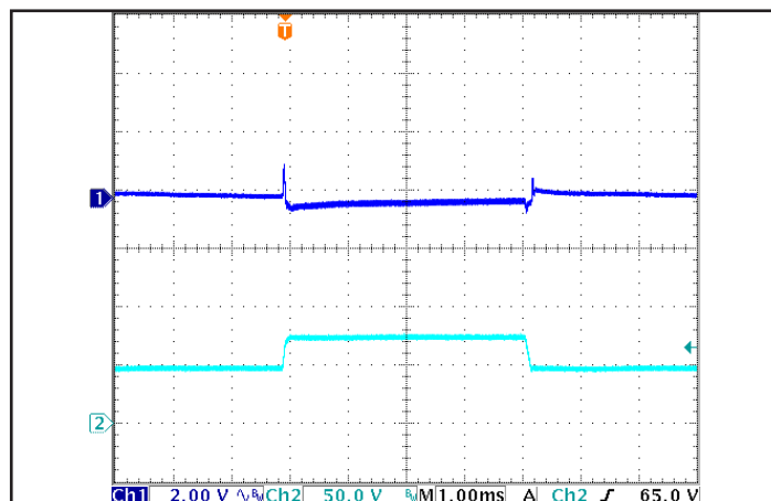
Figure 6: Output Voltage Response to Step-Change in Input Voltage (500 V/ms), at Max. load current. Load cap: 100μF electrolytic cap and 1μF ceramic cap. Ch 1: V out , Ch 2: V in .
