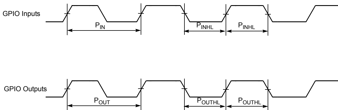
Figure 4-31 GPIO Timing
