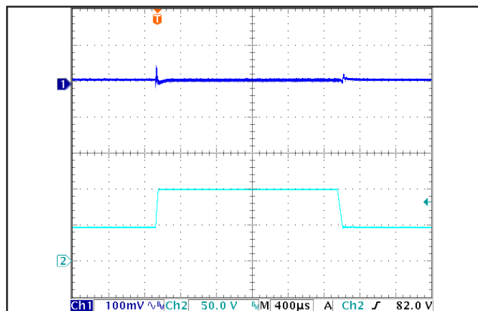
Figure 6: Output voltage response to step-change in input voltage (72V to 100V), at 14A load current. Load cap: 15μF tantalum capacitor and 1μF ceramic cap. Ch 1: Vout (100mV/div), Ch 2: Vin (50V/div).
