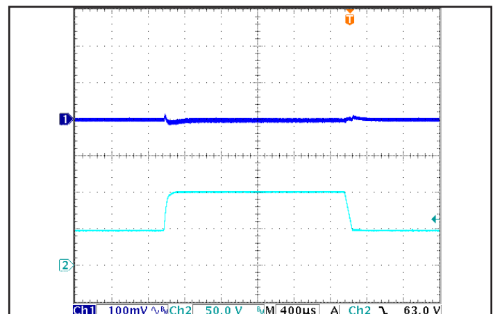
Figure 6: Output voltage response to step-change in input voltage (72V to 100V), at 20A load current. Load cap: 15μF tantalum capacitor and 1μF ceramic cap. Ch 1: Vout (100mV/div), Ch 2: Vin (50V/div).
