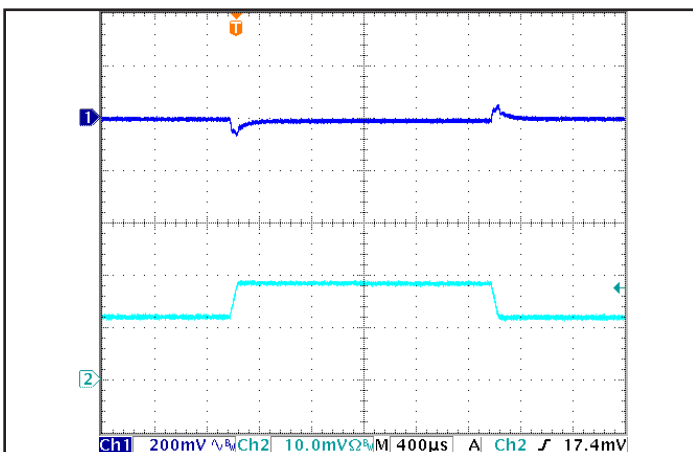
Figure 5: Output voltage response to step-change in load current (66%-100%-66% of Iout(max); dI/dt = 0.1A/μs). Load cap: 15μF tantalum cap and 1μF ceramic cap. Ch 1: Vout (200mV/div), Ch 2: Iout (10A/div).
