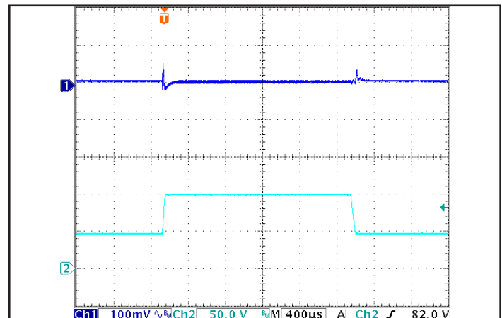
Figure 6: Output voltage response to step-change in input voltage (72V to 100V), at 14A load current. Load cap: 15μF tantalum capacitor and 1μF ceramic cap. Ch 1: V out (100mV/div), Ch 2: V in (50V/div).
