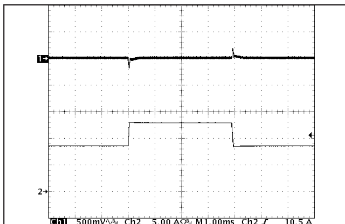
Figure 5: Output voltage response to step-change in load current (50%-75%-50% of Iout(max); dI/dt = 0.1 A/μs). Load cap: 1 μF ceramic and 15 μF tantalum capacitors. Ch 1: Vout, Ch 2: Iout.
