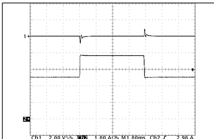
Figure 5: Output voltage response to step-change in load current (50%-75%-50% of I out (max); dI/dt = 0.08 A/μs). Load cap: 1 μF ceramic and 15 μF tantalum capacitors. Ch 1: V out , Ch 2: I out .
