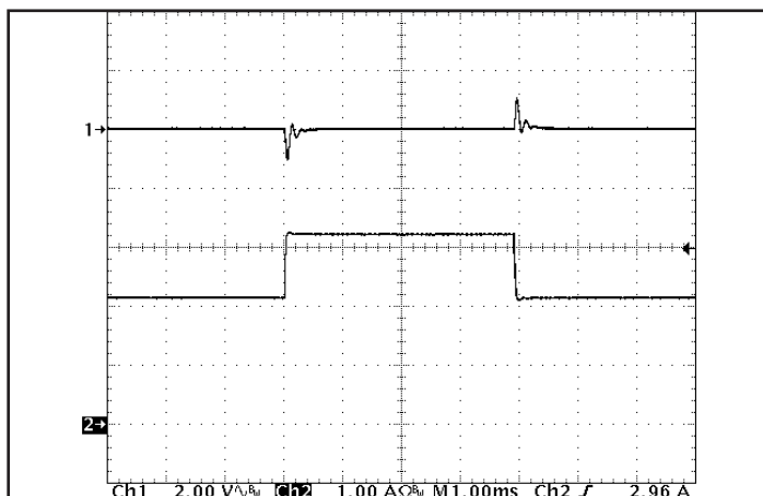
Figure 5: Output voltage response to step-change in load current (50%-75%-50% of Iout(max); dI/dt = 0.05 A/μs). Load cap: 1 μF ceramic and 15 μF tantalum capacitors. Ch 1: Vout, Ch 2: Iout.
