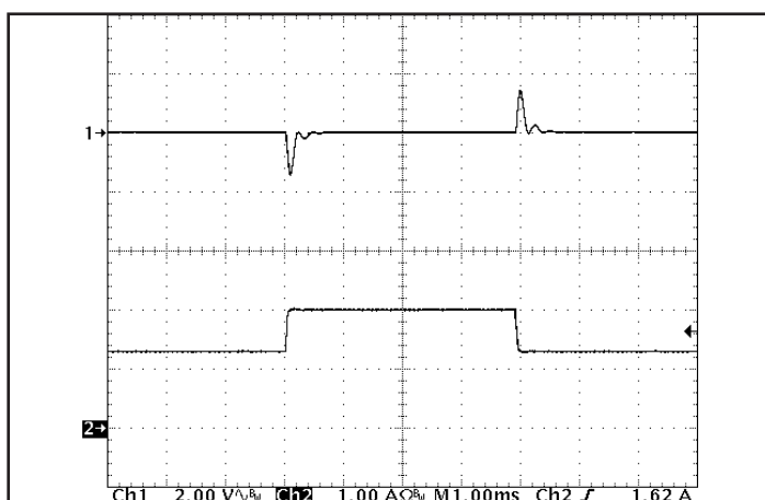
Figure 5: Output voltage response to step-change in load current (50%-75%-50% of I out (max); dI/dt = 0.02 A/μs). Load cap: 1 μF ceramic and 15 μF tantalum capacitors. Ch 1: V out , Ch 2: I out .
