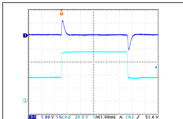
Figure 6: Output voltage response to step-change in input voltage (nominal to maximum, 1000 V/ms). Load cap: 1μF ceramic capacitor. Ch 1: V out , Ch 2: V in .
