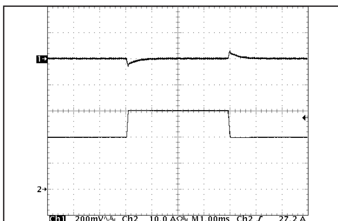
Figure 5: Output voltage response to step-change in load current (66%-100%-66% of I out (max); dI/dt = 0.2 A/μs). Load cap: 1 μF ceramic and 15 μF tantalum capacitors. Ch 1: V out (200 mV/div), Ch 2: I out (10 A/div).
