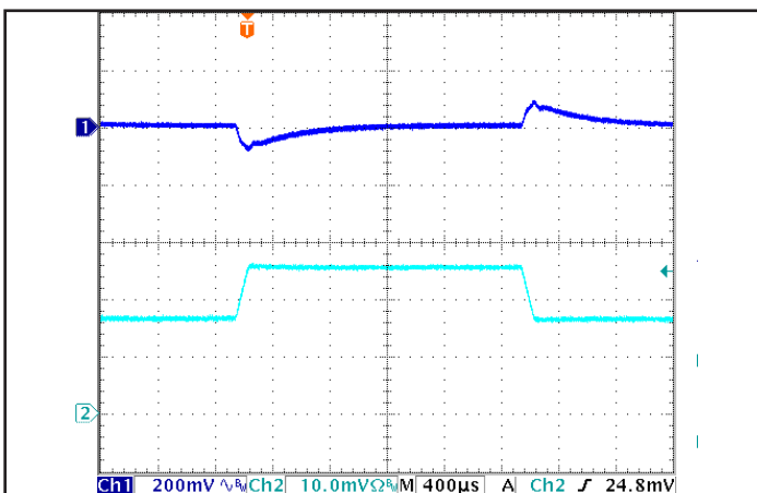
Figure 5: Output voltage response for to step-change in load current (70%-100%-70% of I out (max); dI/dt = 0.6A/μs). Load cap: 15μF tantalum cap and 1μF ceramic cap. Ch 1: V out , Ch 2: I out (10A/div).
