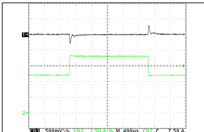
Figure 5: Output voltage response for QTC version of product to step-change in load current (50%-75%-50% of I out (max); dI/dt = 0.6A/μs). Load cap: 15μF tantalum cap and 1μF ceramic cap. Ch 1: V out , Ch 2: I out .
