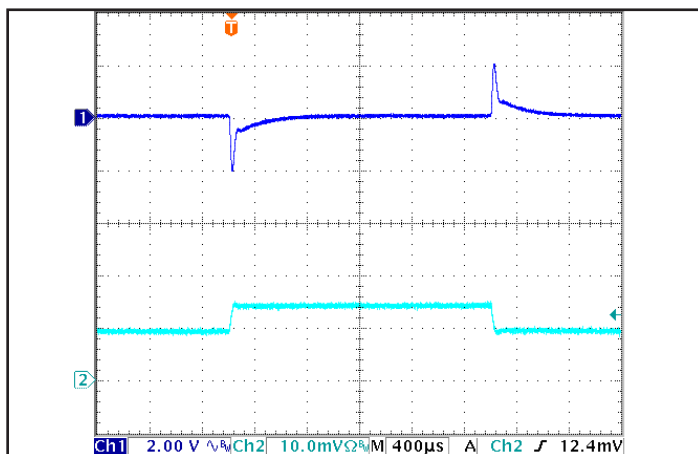
Figure 5: Output voltage response to step-change in load current for QTC version of product (50%-75%-50% of Iout(max); dI/dt = 0.6A/μs). Load cap: 1μF ceramic cap. Ch 1: Vout, Ch 2: Iout (1A/div).
