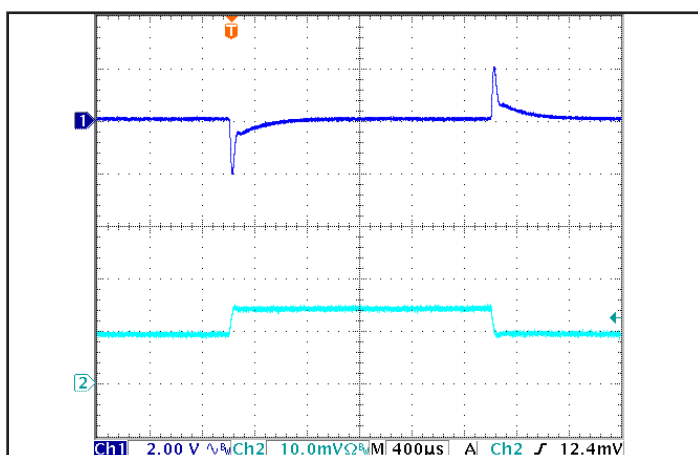
Figure 5: Output voltage response for QTC version of product to step-change in load current (50%-75%-50% of I out (max); dI/dt = 0.6A/μs). Load cap: 1μF ceramic cap. Ch 1: V out , Ch 2: I out (1A/div).
