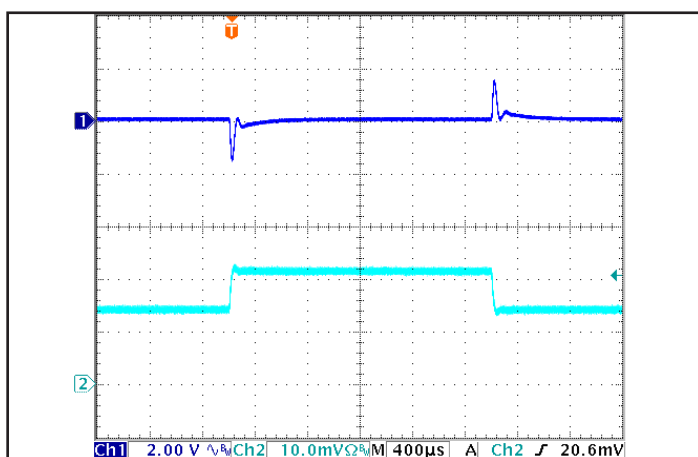
Figure 5: Output voltage response to step-change in load current for QTC version of product (50%-75%-50% of I out (max); dI/dt = 0.6A/μs). Load cap: 1μF ceramic cap. Ch 1: V out , Ch 2: I out (1A/div).
