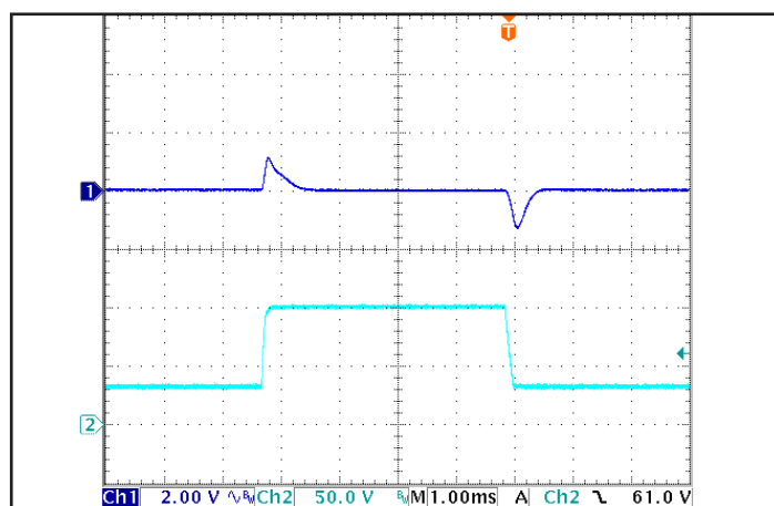
Figure 6: Output voltage response to step-change in input voltage (nominal to maximum), at full load current. Load cap: 1μF ceramic cap. Ch 1: V out , Ch 2: V in .
