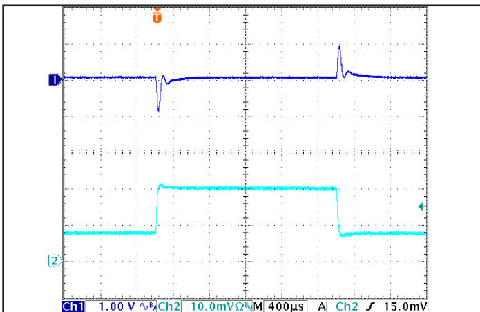
Figure 5: Output voltage response to step-change in load current (50%-75%-50% of I out (max); dI/dt = 0.6A/µs). Load cap: 15µF tantalum cap and 1µF ceramic cap. Ch 1: V out , Ch 2: I out (2A/div).
