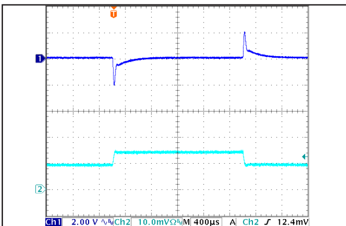
Figure 5: Output voltage response to step-change in load current (50%-75%-50% of Iout(max); dI/dt = 0.6A/us). Load cap: 1uF ceramic cap. Ch 1: Vout, Ch 2: Iout (1A/div).
