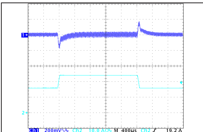
Figure 5: Output voltage response to step-change in load current (66%-100%-66% of Iout(max); dI/dt = 0.1A/us). Load cap: 15µF tantalum cap and 1µF ceramic cap. Ch 1: Vout, Ch 2: Iout.
