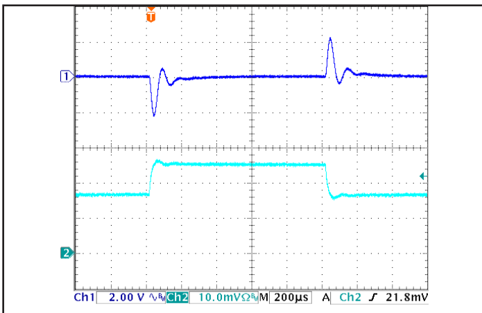
Figure 5: Output voltage response to step-change in load current (66%-100%-66% of Iout(max); dI/dt = 0.1A/µs). Load cap: 1µF ceramic cap. Ch 1: Vout, Ch 2: Iout (1 A/div).
