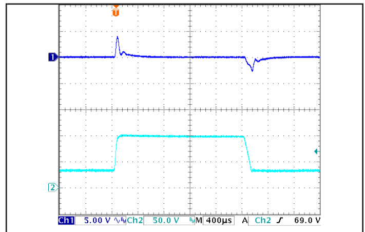
Figure 6: Output voltage response to step-change in input voltage (Vnom.-Vmax.-Vnom.), at Max. load current. Load cap: 1µF ceramic cap. Ch 1: Vout, Ch 2: Vin.
