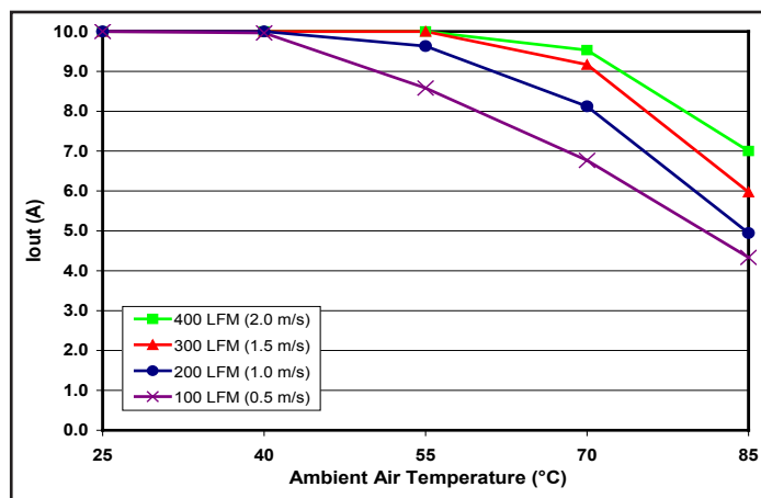
Figure 4: Thermal Derating (max output current vs. ambient air temperature) for encased converter with 1/2" heatsink, at airflow rates of 100 LFM through 400 LFM. Air flows across the converter from input to output (nominal input voltage).
