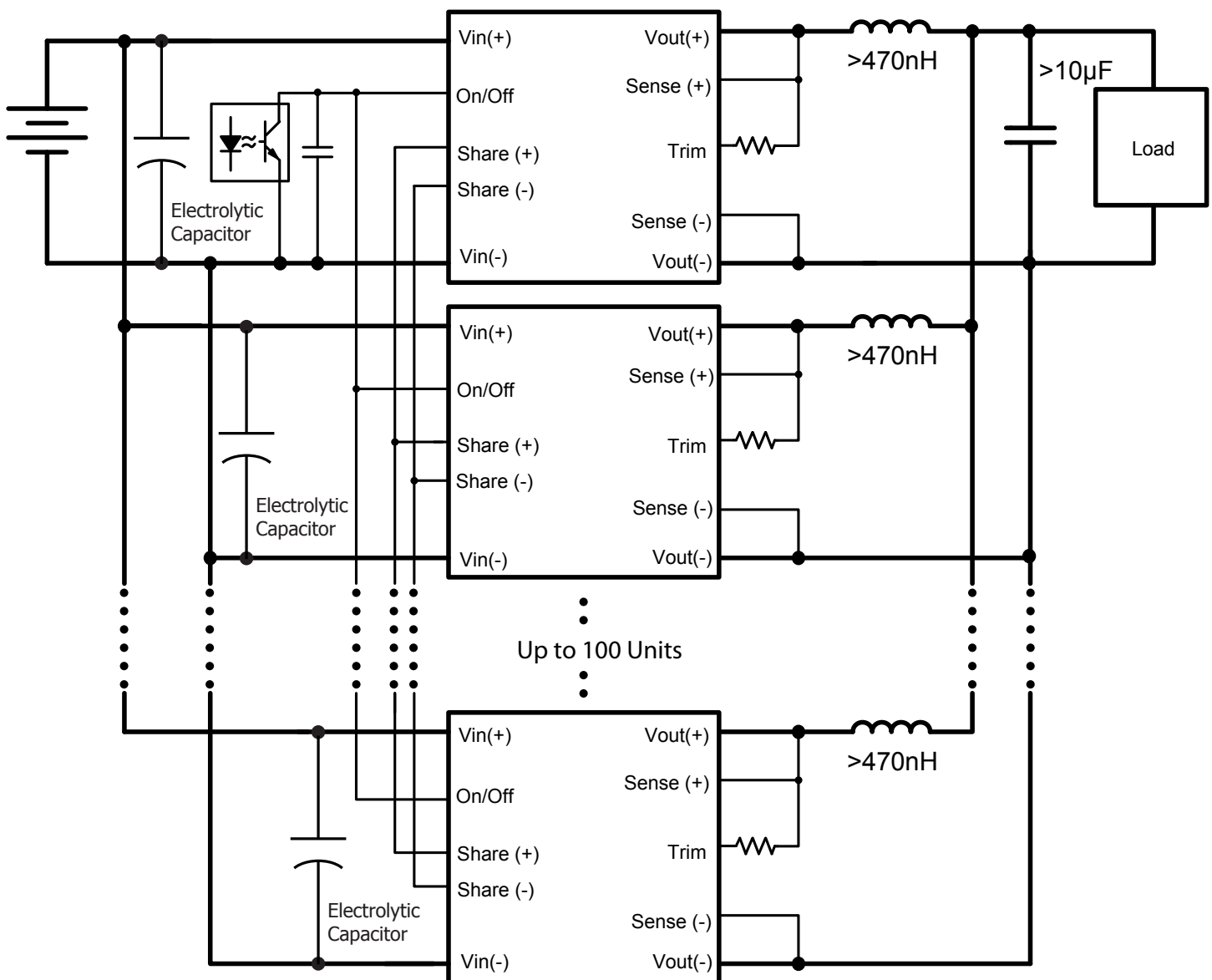
Figure E: Typical Application Circuit for Paralleling of Full-Featured Units
