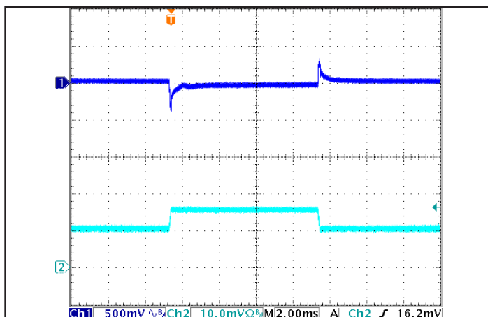
Figure 5: Output Voltage Response to Step-Change in Load Current (50%-75%-50% of I out (max); dI/dt = 0.1A/μs. Load cap: 15μF tantalum cap and 1μF ceramic cap. Ch 1: V out , Ch 2: I out (20 A/div).
