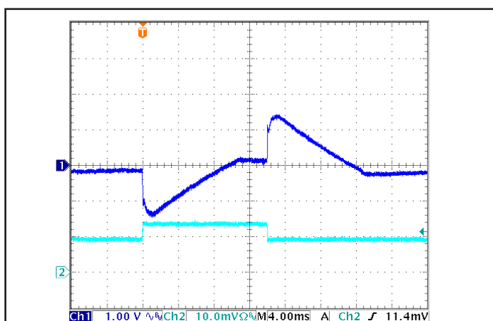
Figure 5: Output Voltage Response to Step-Change in Load Current (50%-75%-50% of I out (max); dI/dt = 0.1A/μs. Load cap: 100μF electrolytic cap and 1μF ceramic cap. Ch 1: V out , Ch 2: I out (10 A/div).
