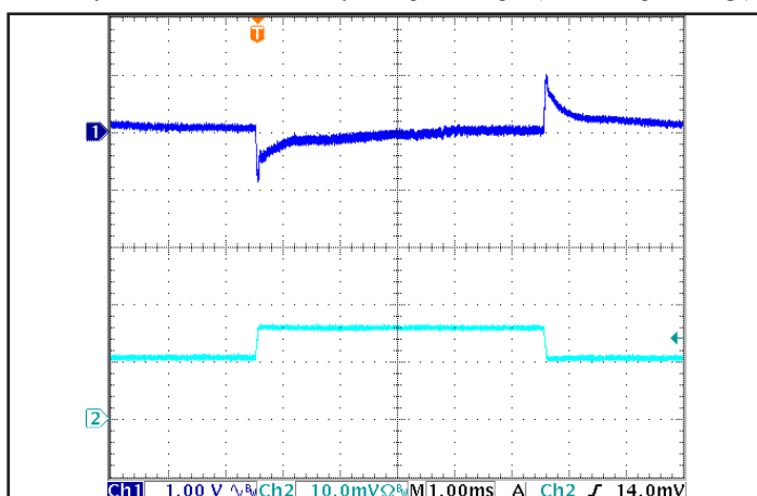
Figure 5: Output Voltage Response to Step-Change in Load Current (50%-75%-50% of I out (max); dI/dt = 0.1A/μs. Load cap: 1μF ceramic cap. Ch 1: V out , Ch 2: I out (10 A/div).
