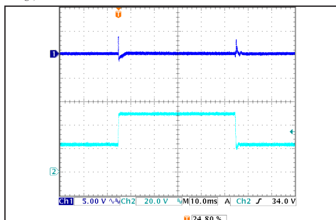
Figure 6: Output Voltage Response to Step-Change in Input Voltage (250 V/ms), at Max. load current. Load cap: 100μF electrolytic cap and 1μF ceramic cap. Ch 1: V out , Ch 2: V in .
