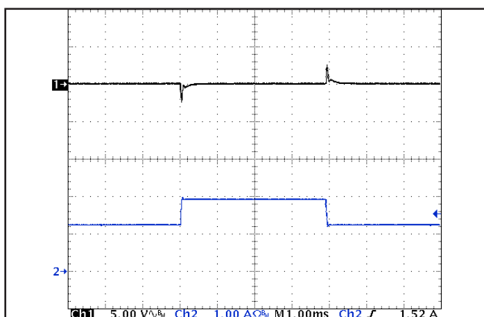
Figure 5: Output voltage response to step-change in load current (50%-75%-50% of I out (max); dI/dt = 0.2A/μs). Load cap: 1μF ceramic cap. Ch 1: V out , Ch 2: I out (1A/div).
