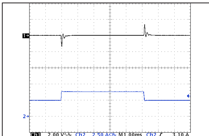
Figure 5: Output voltage response to step-change in load current (66%-100%-66% of I out (max); dI/dt = 0.05 A/μs). Load cap: 1 μF ceramic capacitor. Ch 1: V out (2 V/div), Ch 2: I out (2.5 A/div).
