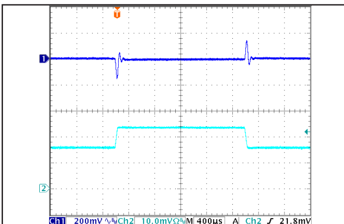
Figure 5: Output voltage response in the SM version to step-change in load current (50%-75%-50% of Iout(max)); di/dt = 0.1 \text{ A}/\mu\text{s} . Load cap: 100 \mu\text{F} electrolytic cap and 1 \mu\text{F} ceramic cap. Ch 1: Vout (200 mV/div), Ch 2: Iout (5 A/div).
