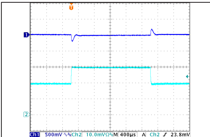
Figure 5: Output voltage response in the SM version to step-change in load current (50%-75%-50% of Iout(max); dI/dt = 0.1 A/µs). Load cap: 100 µF electrolytic cap and 1 µF ceramic cap. Ch 1: Vout (500 mV/div), Ch 2: Iout (1 A/div).
