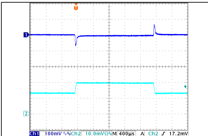
Figure 5: Output voltage response in the SM version unit to step-change in load current (50%-75%-50% of Iout(max)); di/dt = 0.1 \text{ A}/\mu\text{s} . Load cap: 100 \mu\text{F} electrolytic cap and 1 \mu\text{F} ceramic cap. Ch 1: Vout (100 mV/div), Ch 2: Iout (10 A/div).
