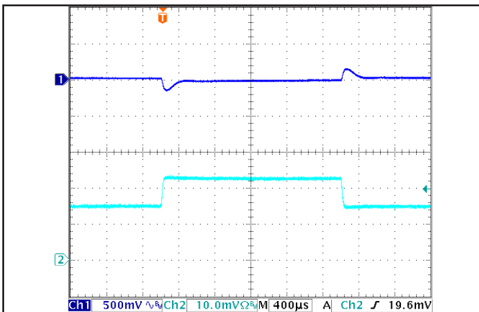
Figure 5: Output voltage response in the SM version to step-change in load current (50%-75%-50% of I out (max); dI/dt = 0.1 A/μs). Load cap: 100 μF electrolytic cap and 1 μF ceramic cap. Ch 1: V out (500 mV/div), Ch 2: I out (1 A/div).
