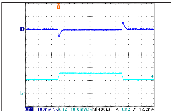
Figure 5: Output voltage response to step-change in load current (50%-75%-50% of I out (max); dI/dt = 0.1 A/μs). Load cap: 100 μF electrolytic cap and 1 μF ceramic cap. Ch 1: V out (100 mV/div), Ch 2: I out (10 A/div).
