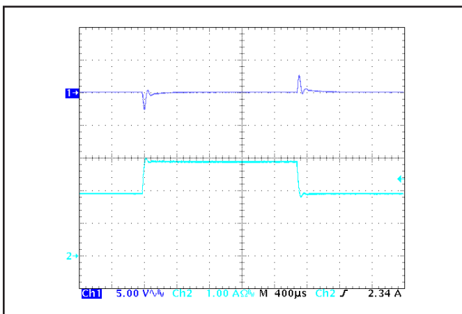
Figure 5: Output voltage response to step-change in load current (50%-75%-50% of I out (max); dI/dt = 0.1 A/µs). Load cap: 1 µF ceramic capacitor. Ch 1: V out (5 V/div), Ch 2: I out (1 A/div).
