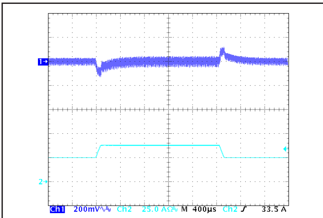
Figure 5: Output voltage response to step-change in load current (50%-75%-50% of Iout(max)); di/dt = 0.1 \text{ A}/\mu\text{s} . Load cap: 1 \mu\text{F} ceramic capacitor. Ch 1: Vout (200 mV/div), Ch 2: Iout (25 A/div).
