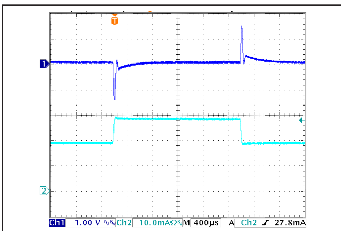
Figure 5: Output voltage response to step-change in load current (50%-75%-50% of Iout(max); dl/dt = 0.1 A/µs). Load cap: 1 µF ceramic capacitor. Ch 1: Vout (1 V/div), Ch 2: Iout (10 mA/div).
