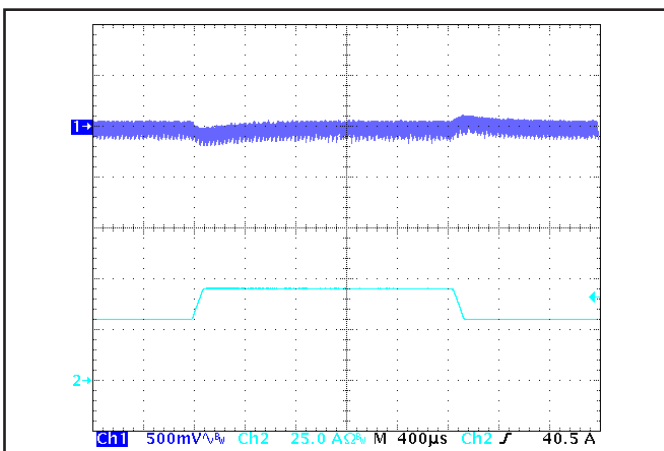
Figure 5: Output voltage response to step-change in load current (50%-75%-50% of Iout(max)); di/dt = 0.1 \text{ A}/\mu\text{s} . Load cap: 1 \mu\text{F} ceramic capacitor. Ch 1: Vout (500 mV/div), Ch 2: Iout (25 A/div).
