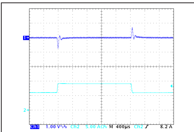
Figure 5: Output voltage response to step-change in load current (50%-75%-50% of Iout(max)); dl/dt = 0.1 A/us. Load cap: 1 μF ceramic capacitor. Ch 1: Vout (1 V/div), Ch 2: Iout (5 A/div).
