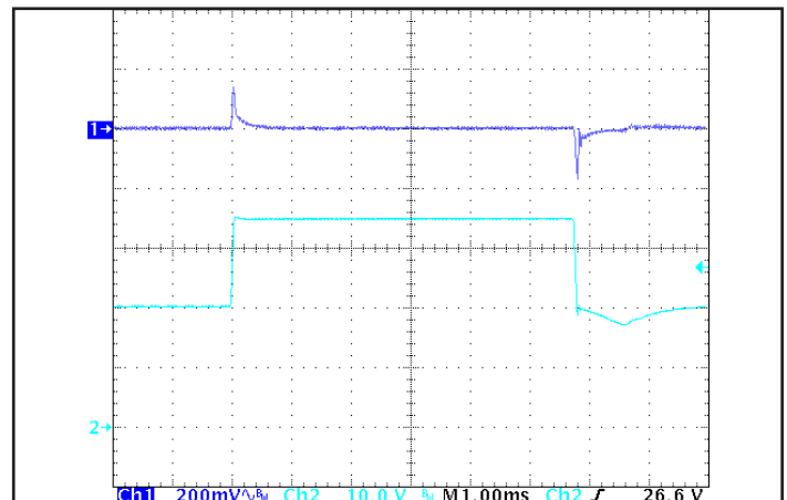
Figure 6: Output voltage response to step-change in input voltage (1000 V/ms). Load cap: 100 µF, electrolytic output capacitance. Ch 1: V out (200 mV/div), Ch 2: V in (10 V/div).
