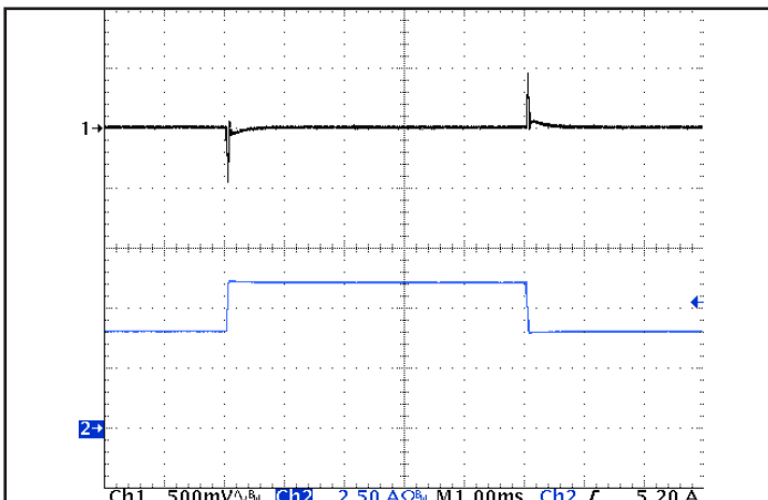
Figure 5: Output voltage response to step-change in load current (50%-75%-50% of I out (max); dI/dt = 0.1 A/μs). Load cap: 1 μF ceramic and 15 μF tantalum capacitors. Ch 1: V out (500 mV/div), Ch 2: I out (2.5 A/div).
