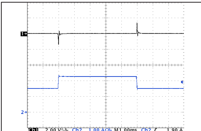
Figure 5: Output voltage response to step-change in load current (50%-75%-50% of Iout(max); dI/dt = 0.05 A/us). Load cap: 1 µF ceramic capacitor. Ch 1: Vout (2 V/div), Ch 2: Iout (1 A/div).
