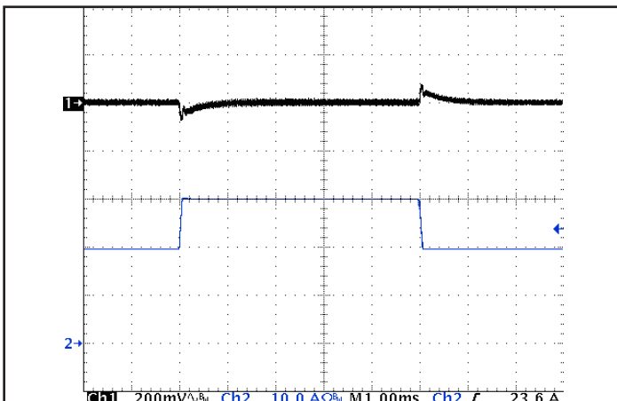
Figure 5: Output voltage response to step-change in load current (50%-75%-50% of I out (max); dI/dt = 0.2A/μs). Load cap: 15μF tantalum cap and 1μF ceramic cap. Ch 1: (200mV/div, Ch 2: I out (10A/div).
