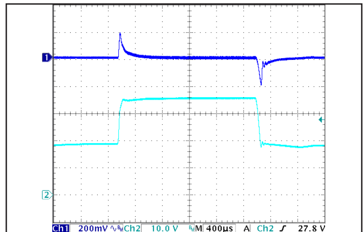
Figure 6: Output voltage response to step-change in input voltage (300 V/ms). Load cap: 100 \mu F , electrolytic output capacitance. Ch 1: Vout (200 mV/div), Ch 2: Vin (10 V/div).
