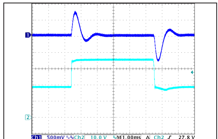
Figure 6: Output voltage response to step-change in input voltage (300 V/ms). Load cap: 100 µF, electrolytic output capacitance. Ch 1: Vout (500 mV/div), Ch 2: Vin (10 V/div).
