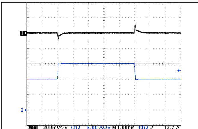
Figure 5: Output voltage response to step-change in load current (50%-75%-50% of Iout(max)); di/dt = 0.1A/\mu s . Load cap: 15 \mu F tantalum cap and 1 \mu F ceramic cap. Ch 1: Vout (200 mV/div), Ch 2: Iout (5 A/div).
