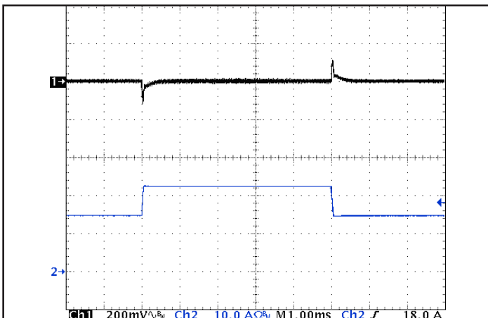
Figure 5: Output voltage response to step-change in load current (50%-75%-50% of I out (max)); dI/dt = 0.2A/μs. Load cap: 15μF tantalum cap and 1μF ceramic cap. Ch 1: V out (200 mV/div), Ch 2: I out (10 A/div).
