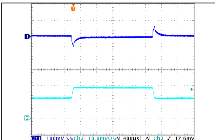
Figure 5: Output voltage response in the SM version to step-change in load current (50%-75%-50% of Iout(max); dI/dt = 0.1 A/µs). Load cap: 100 µF electrolytic cap and 1 µF ceramic cap. Ch 1: Vout (100 mV/div), Ch 2: Iout (10 A/div).
