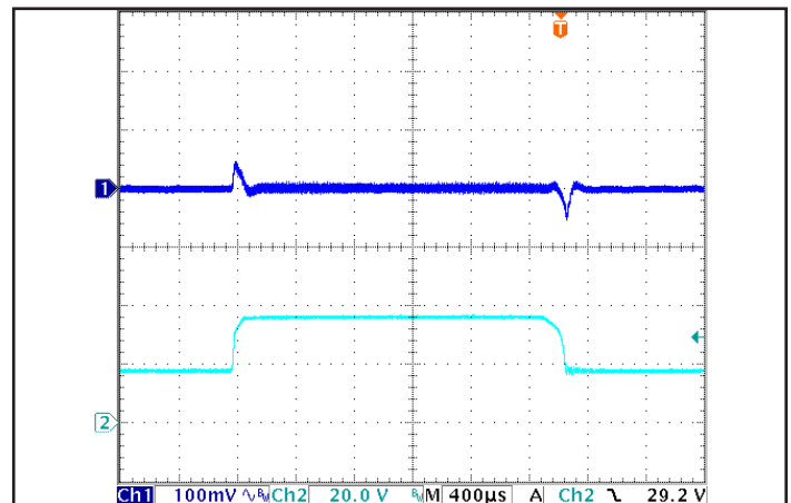
Figure 6: Output voltage response in the SM version to step-change in input voltage (250 V/ms). Load cap: 100 \mu\text{F} electrolytic output capacitance. Ch 1: Vout (100 mV/div), Ch 2: Vin (20 V/div).
