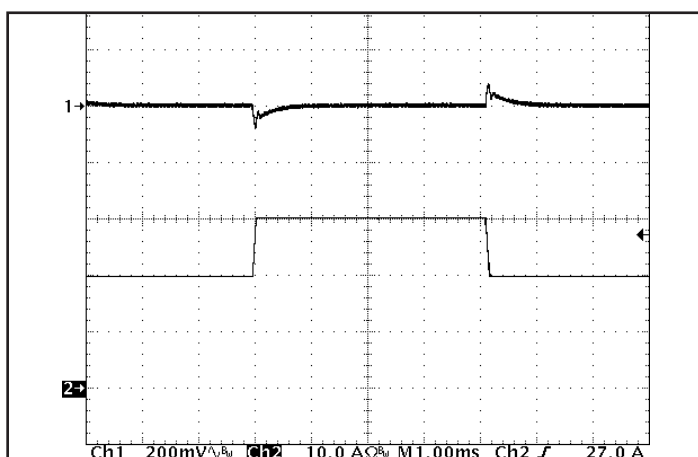
Figure 5: Output voltage response to step-change in load current (66%-100%-66% of I out (max); dI/dt = 0.2A/μs). Load cap: 1μF ceramic cap and 15μF tantalum cap. Ch 1: V out (200mV/div), Ch 2: I out (10A/div).
