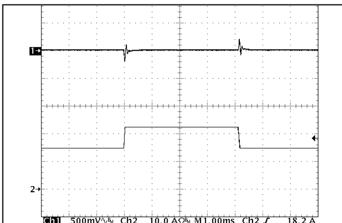
Figure 5: Output voltage response to step-change in load current (66%-100%-66% of Iout(max); dI/dt = 0.2A/μs). Load cap: 15μF tantalum cap and 1μF ceramic cap. Ch 1: Vout (500mV/div), Ch 2: Iout (10A/div).
