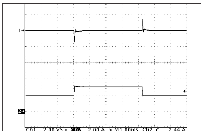
Figure 5: Output voltage response to step-change in load current (66%-100%-66% of I out (max); dI/dt = 0.08A/μs). Load cap: 1μF ceramic cap. Ch 1: V out (2V/div), Ch 2: I out (2A/div).
