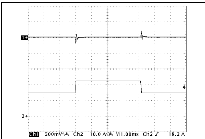
Figure 5: Output voltage response to step-change in load current (50%-75%-50% of I out (max)); dI/dt = 0.2 A/μs. Load cap: 1 μF ceramic and 15 μF tantalum capacitors. Ch 1: V out (500 mV/div), Ch 2: I out (10 A/div).
