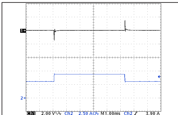
Figure 5: Output voltage response to step-change in load current (66%-100%-66% of I out (max); dI/dt = 0.1 A/μs). Load cap: 1 μF ceramic capacitor. Ch 1: V out (2 V/div), Ch 2: I out (2.5 A/div).
