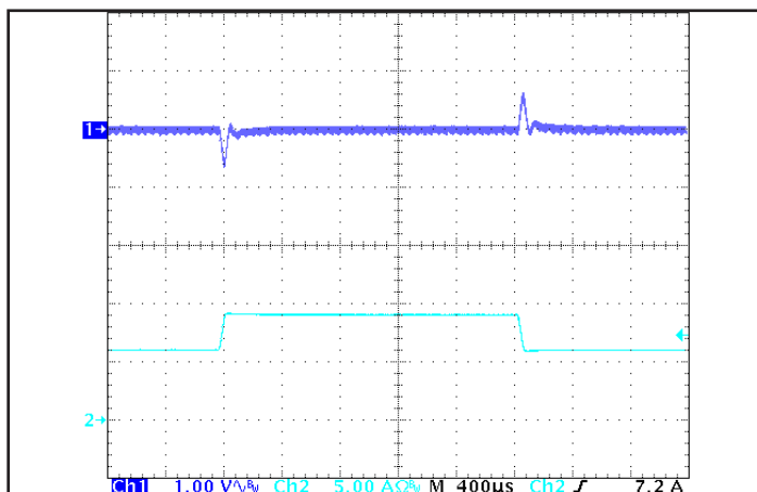
Figure 5: Output voltage response to step-change in load current (66%-100%-66% of Iout(max); dI/dt = 0.1 A/μs). Load cap: 1 μF ceramic and 15 μF tantalum capacitors. Ch 1: Vout (1 V/div), Ch 2: Iout (5 A/div).
