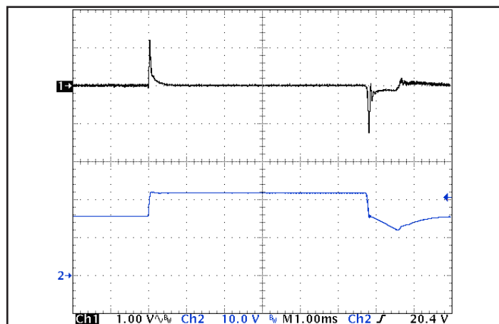
Figure 6: Output voltage response to step-change in input voltage (500 V/ms). Load cap: 100 μF, electrolytic output capacitance. Ch 1: Vin (1 V/div), Ch 2: Vout (10 V/div).
