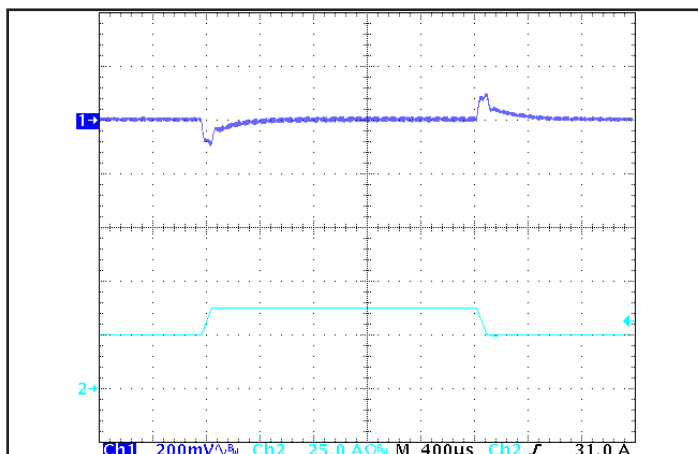
Figure 5: Output voltage response to step-change in load current (66%-100%-75% of I out (max); dI/dt = 0.2 A/μs). Load cap: 1 μF ceramic and 15 μF tantalum capacitors. Ch 1: V out (200 mV/div), Ch 2: I out (25 A/div).
