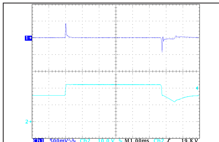
Figure 6: Output voltage response to step-change in input voltage (500 V/ms). Load cap: 100 μF, electrolytic output capacitance. Ch 1: Vout (500 mV/div), Ch 2: Vin (10 V/div).
