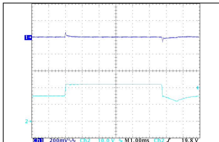
Figure 6: Output voltage response to step-change in input voltage (500 V/ms). Load cap: 100 μF, electrolytic output capacitance. Ch 1: Vout (200 mV/div), Ch 2: Vin (10 V/div).
