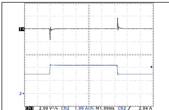
Figure 5: Output voltage response to step-change in load current (50%-75%-50% of Iout(max); dI/dt = 0.1A/us). Load cap: 1uF ceramic cap. Ch 1: Vout, Ch 2: Iout.
