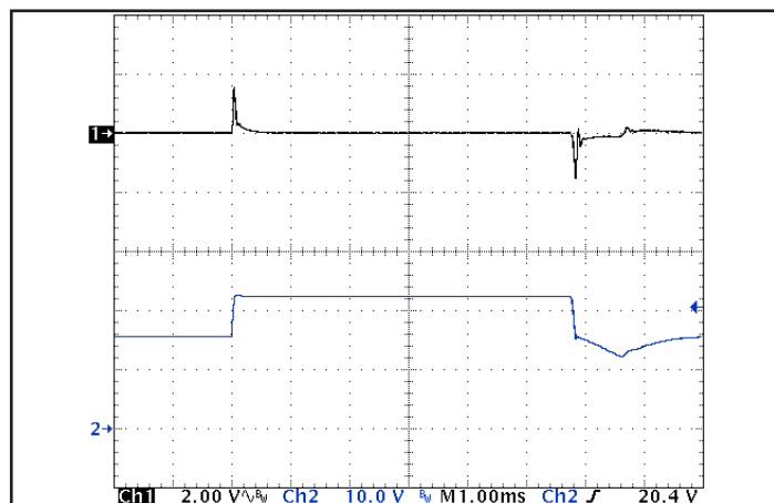
Figure 6: Output voltage response to step-change in input voltage (Vnom.-Vmax-Vnom.), at Max. load current. Load cap: 1uF ceramic cap. Ch 1: Vout, Ch 2: Vin.
