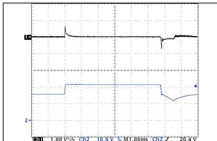
Figure 6: Output voltage response to step-change in input voltage ( V_{nom.} - V_{max} - V_{nom.} ), at Max. load current. Load cap: 1 \mu F ceramic cap. Ch 1: V_{out} , Ch 2: V_{in} .
