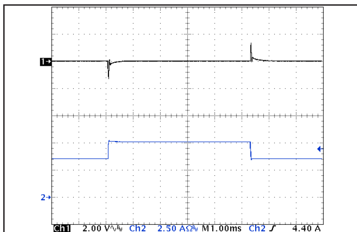
Figure 5: Output voltage response to step-change in load current (50%-75%-50% of I_{out(max)} ; dI/dt = 0.1A/\mu s ). Load cap: 1 \mu F ceramic cap. Ch 1: V_{out} , Ch 2: I_{out} .
