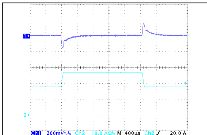
Figure 5: Output voltage response to step-change in load current (50%-75%-50% of I_{out(max)} ; dI/dt = 0.1A/\mu s ). Load cap: 15μF tantalum cap and 1μF ceramic cap. Ch 1: Vout, Ch 2: Iout.
