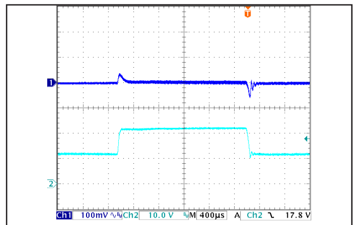
Figure 6: Output voltage response in SM version to step-change in input voltage (250 V/ms). Load cap: 100 \mu\text{F} electrolytic output capacitance. Ch 1: Vout (100 mV/div), Ch 2: Vin (10 V/div).
