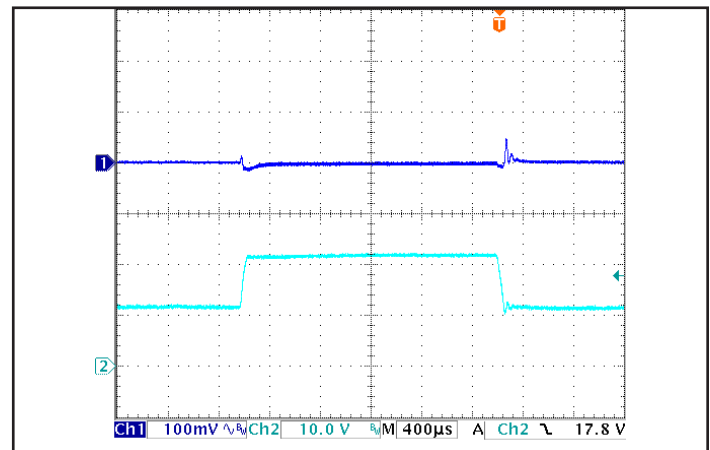
Figure 6: Output voltage response in SM version to step-change in input voltage (250 V/ms). Load cap: 100 μF, electrolytic output capacitance. Ch 1: Vout (100 mV/div), Ch 2: Vin (10 V/div).
