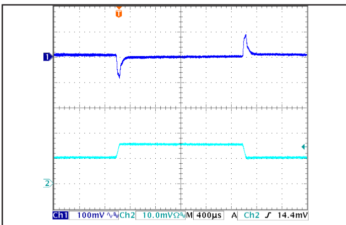
Figure 5: Output voltage response for Mega version of the unit to step-change in load current (50%-75%-50% of Iout(max); di/dt = 0.1 \text{ A}/\mu\text{s} ). Load cap: 100 \mu\text{F} electrolytic cap and 1 \mu\text{F} ceramic cap. Ch 1: Vout (100 mV/div), Ch 2: Iout (10 A/div).
