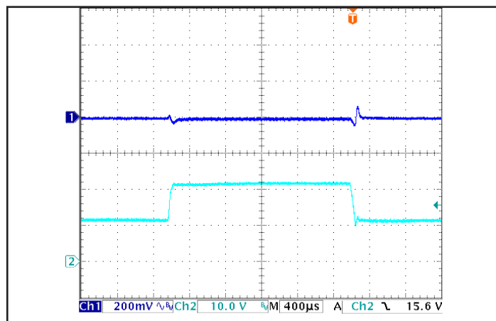
Figure 6: Output voltage response in SM version to step-change in input voltage (250 V/ms). Load cap: 100 \mu\text{F} electrolytic output capacitance. Ch 1: Vout (200 mV/div), Ch 2: Vin (10 V/div).
