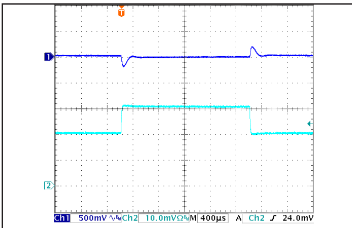
Figure 5: Output voltage response for Mega version of the unit to step-change in load current (50%-75%-50% of Iout(max); dI/dt = 0.1 A/μs). Load cap: 100 μF electrolytic cap and 1 μF ceramic cap. Ch 1: Vout (500 mV/div), Ch 2: Iout (1 A/div).
