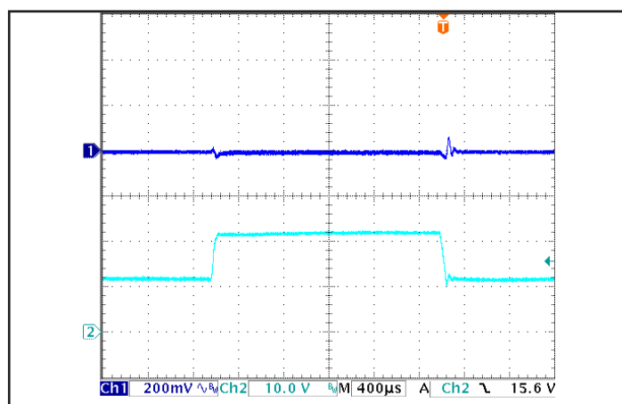
Figure 6: Output voltage response in SM version for Mega version of the unit to step-change in input voltage (250 V/ms). Load cap: 100 μF electrolytic output capacitance. Ch 1: Vout (200 mV/div), Ch 2: Vin (10 V/div).
