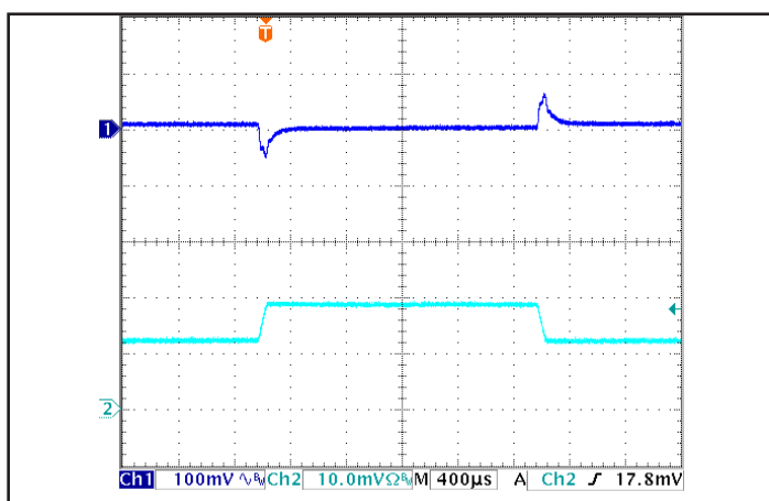
Figure 5: Output voltage response to step-change in the SM version to load current (65%-95%-65% of Iout(max); dI/dt = 0.1 A/μs). Load cap: 100 μF electrolytic cap and 1 μF ceramic cap. Ch 1: Vout (100 mV/div), Ch 2: Iout (10 A/div).
