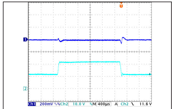
Figure 6: Output voltage in SM version response to step-change in input voltage (250 V/ms). Load cap: 100 μF, electrolytic output capacitance. Ch 1: Vout (200 mV/div), Ch 2: Vin (10 V/div).
