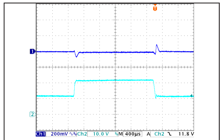
Figure 6: Output voltage response in SM version to step-change in input voltage (250 V/ms). Load cap: 100 μF, electrolytic output capacitance. Ch 1: Vout (200 mV/div), Ch 2: Vin (10 V/div).
