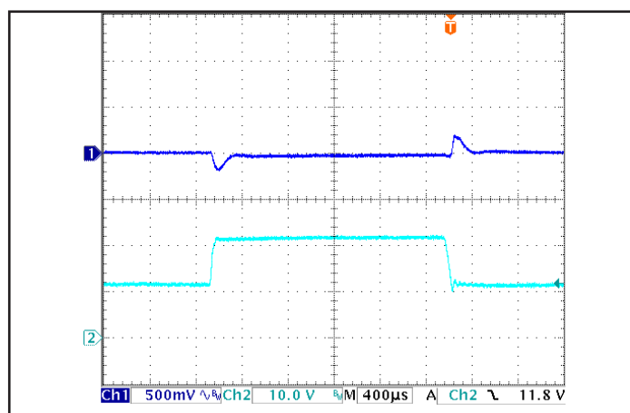
Figure 6: Output voltage response in SM version to step-change in input voltage (250 V/ms). Load cap: 100 μF, electrolytic output capacitance. Ch 1: Vout (500 mV/div), Ch 2: Vin (10 V/div).
