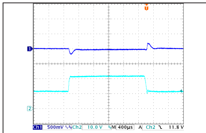
Figure 6: Output voltage response to step-change in input voltage (250 V/ms). Load cap: 100 μF, electrolytic output capacitance. Ch 1: Vout (500 mV/div), Ch 2: Vin (10 V/div).
