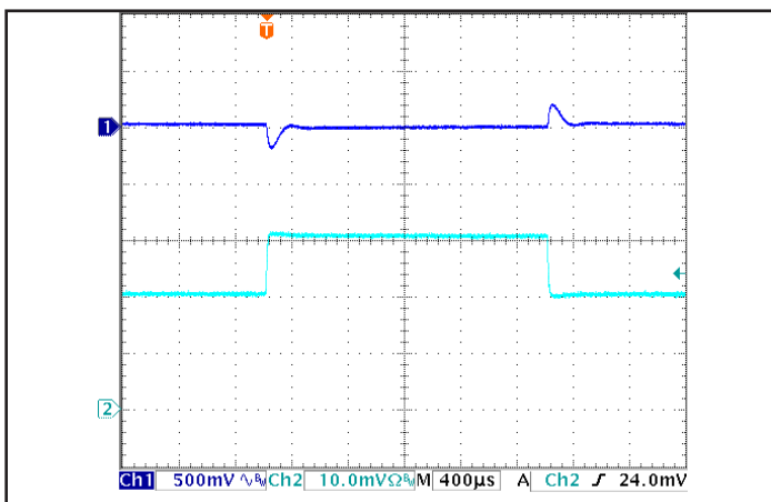
Figure 5: Output voltage response to step-change in load current (50%-75%-50% of I out(max) ; dI/dt = 0.1 A/μs). Load cap: 100 μF electrolytic cap and 1 μF ceramic cap. Ch 1: V out (500 mV/div), Ch 2: I out (1 A/div).
