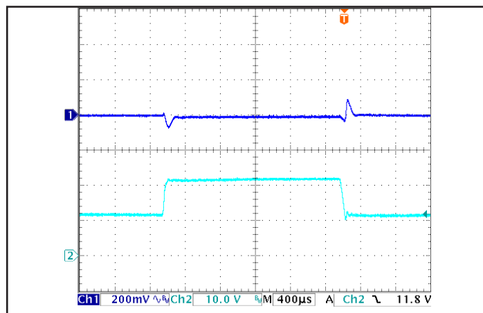
Figure 6: Output voltage response to step-change in input voltage (250 V/ms). Load cap: 100 μF, electrolytic output capacitance. Ch 1: Vout (200 mV/div), Ch 2: Vin (10 V/div).
