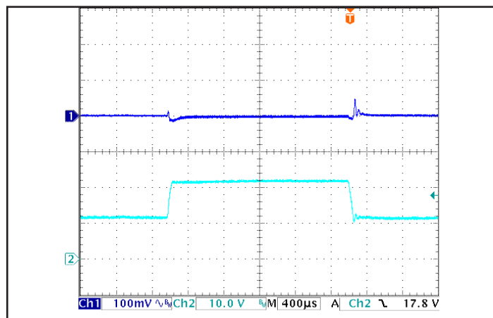
Figure 6: Output voltage response to step-change in input voltage (250 V/ms). Load cap: 100 μF, electrolytic output capacitance. Ch 1: Vout (100 mV/div), Ch 2: Vin (10 V/div).
